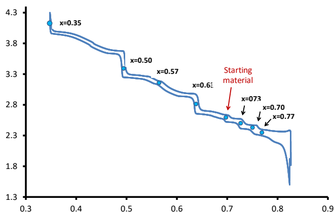
Figure 20. Electrochemical cycling of a Na // P2- \text{Na}_x\text{CoO}_2 battery.
