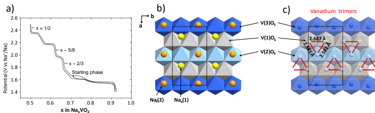
Figure 21. Electrochemical cycling of a Na // P2- \text{Na}_x\text{VO}_2 battery (a). Structure of the \text{Na}_{1/2}\text{VO}_2 phase obtained by electrochemical deintercalation: sodium ordering in the Na layer (b), formation of vanadium trimers in the \text{VO}_2 slab (c). Adapted with permission Guignard M., Didier C. et al., Nat. Mater. 2013, 12 , 74 Copyright 2020, Nature.
