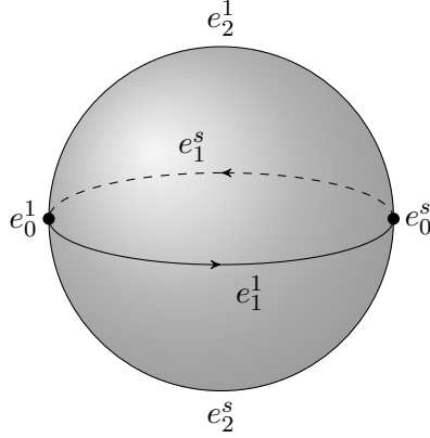
FIGURE 5. Equivariant cellular decomposition of \mathrm{SU}(2)/T = \mathbb{S}^2 .
