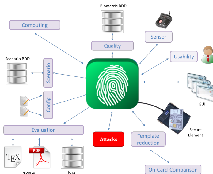
Figure 4. General diagram of the EvaBio platform (defined in [16]).
