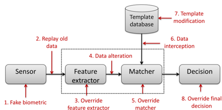
Figure 1. Locating vulnerabilities on a biometric system (defined by [2]).
