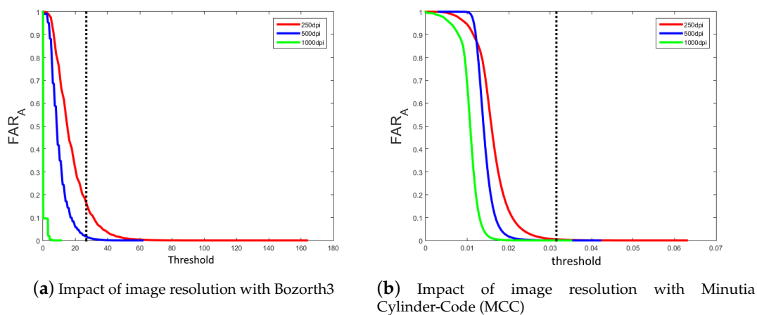
Figure 5. Evolution of the effectiveness of attacks by considering the three resolutions of the sensor for the two matching algorithms. The dot line corresponds to the threshold value associated to the Equal Error Rate (EER) performance (see Section 2.1.2).
