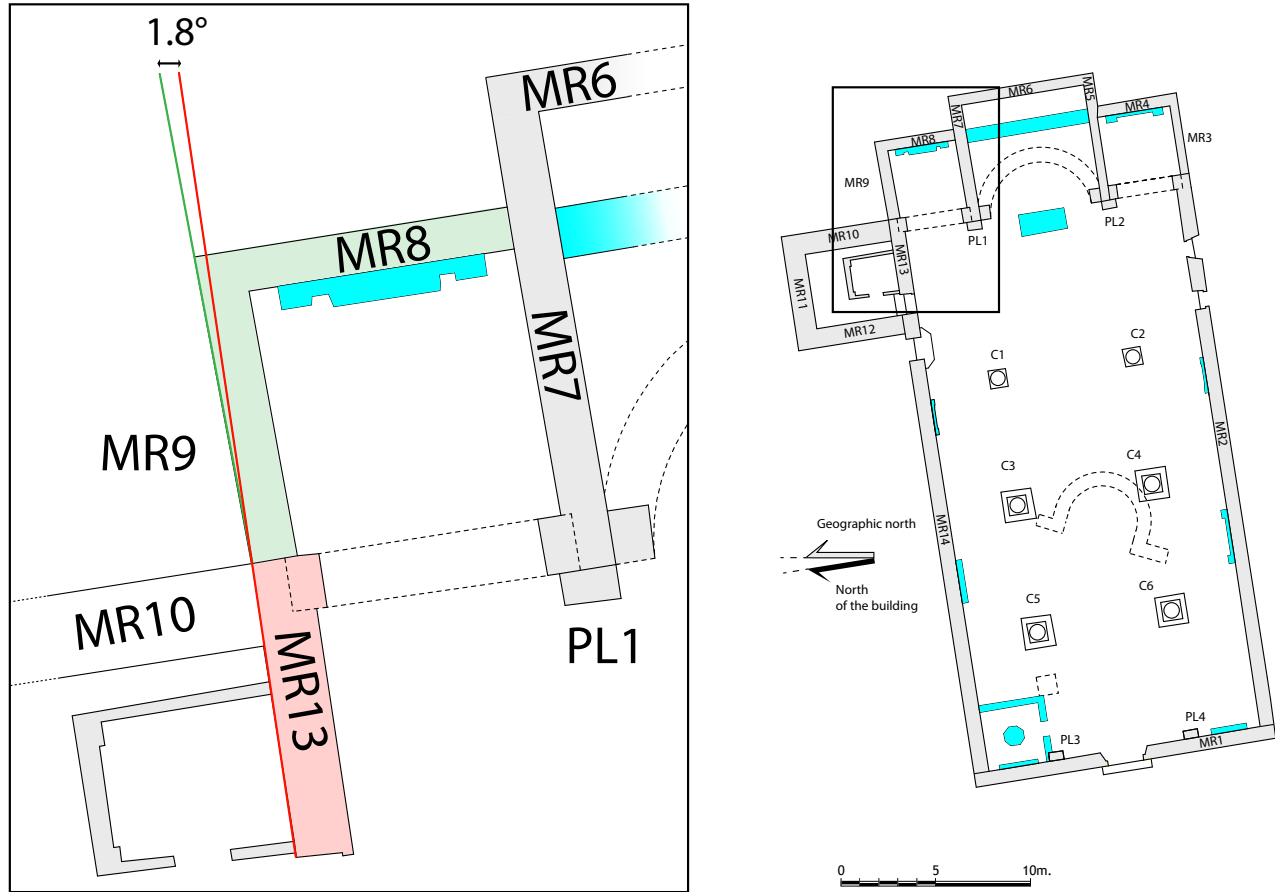
Figure 15: Zoom in the northeast lateral apse. A misalignment is observed between MR9 and MR13.
