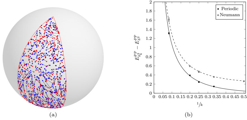
FIGURE 7. (a) Optimal assignment on a spherical lune. (b) Comparison between numerical results and our theoretical prediction for E_{S_k}^{\text{PP}} - E_{S^2}^{\text{PP}} with periodic (smooth line) and Neumann (dashed line) boundary conditions.
