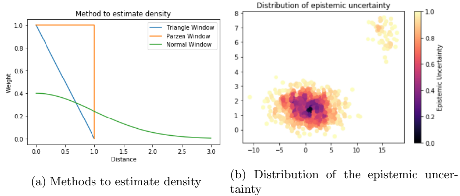
Fig. 2: Epistemic uncertainty
