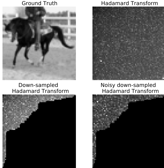
Fig. 1. An image from the stl-10 dataset, alongside its Hadamard transform, the Hadamard transform with missing coefficients (down-sampled Hadamard transform), and the Hadamard transform with missing coefficients (noisy down-sampled Hadamard transform). The noisy coefficients are subject to Poison noise, and we chose \alpha = 10 ph.
