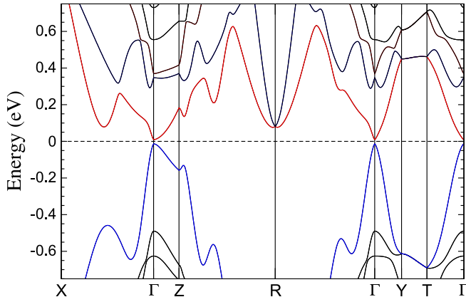
FIG. 1. Ab initio calculated band structure of \text{ZrTe}_5 . The valence and the conduction bands are drawn in blue and red, respectively.
