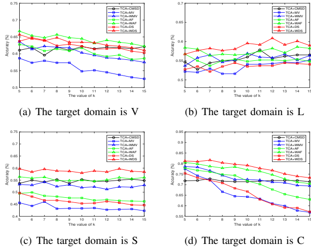
Fig. 3. Classification accuracy of different methods based on TCA and k -NN classifier with tuning of k values.
