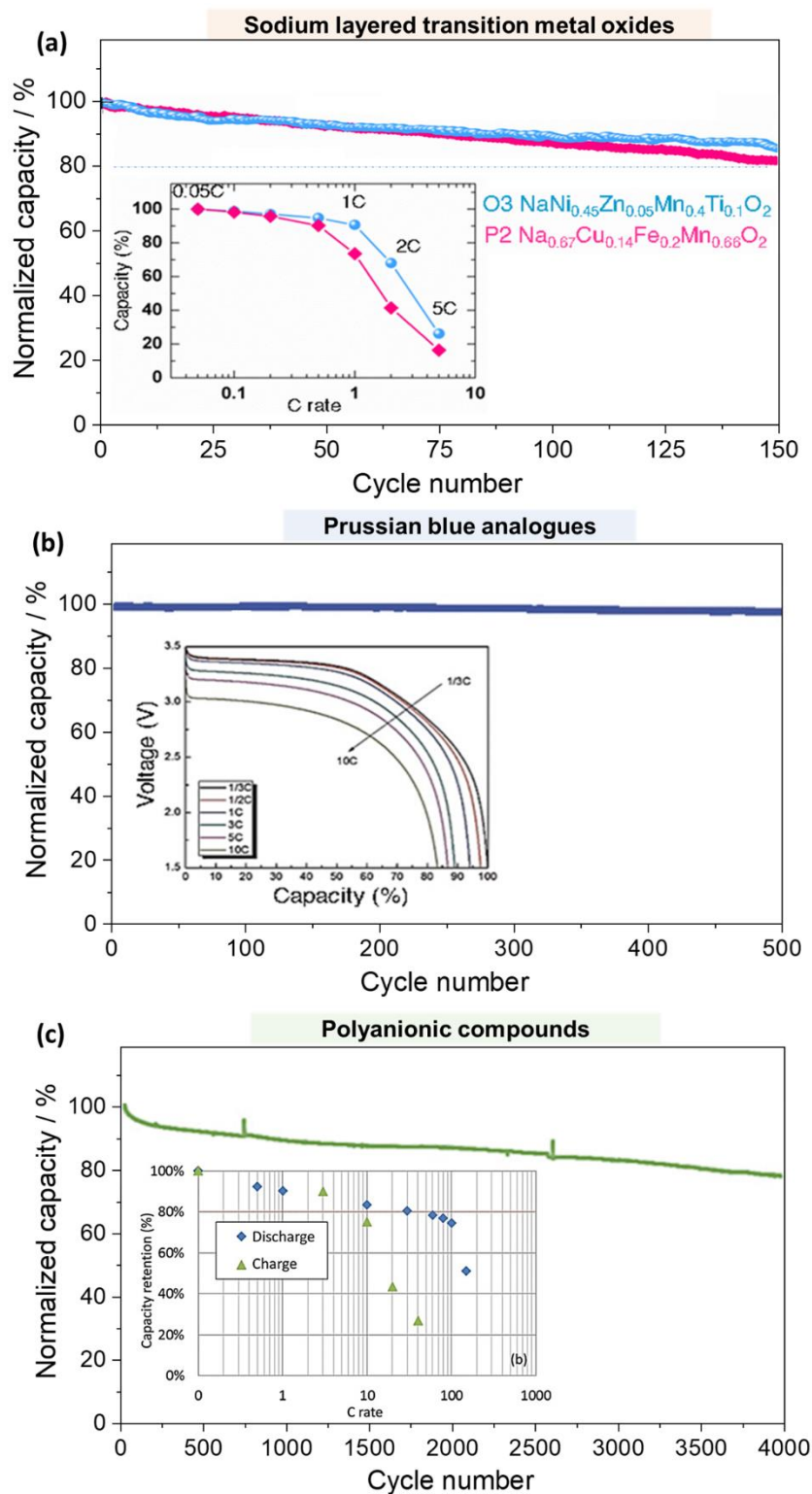
Figure 3: Comparison of cycle life (capacity retention) and power rate capability of three different families of positive electrodes. (a) Sodium layered oxides O3 \text{NaNi}_{0.45}\text{Zn}_{0.05}\text{Mn}_{0.4}\text{Ti}_{0.1}\text{O}_2 (100% capacity= 145 \text{mAh.g}^{-1} ) and P2 \text{Na}_{0.67}\text{Cu}_{0.14}\text{Fe}_{0.2}\text{Mn}_{0.66}\text{O}_2 (100% capacity= 103 \text{mAh.g}^{-1} ) cycled in coin cell at C/10 rate using hard carbon as negative electrode and 1M \text{NaPF}_6 in propylene carbonate as electrolyte. Inset shows the power rate capability of the materials tested in Na-half cells using sodium metal as counter and negative electrode. The capacity of 172 and 255 \text{mAh.g}^{-1} are taken as 100% capacity for O3 and P2 layered oxides respectively. (b) Prussian blue analog
