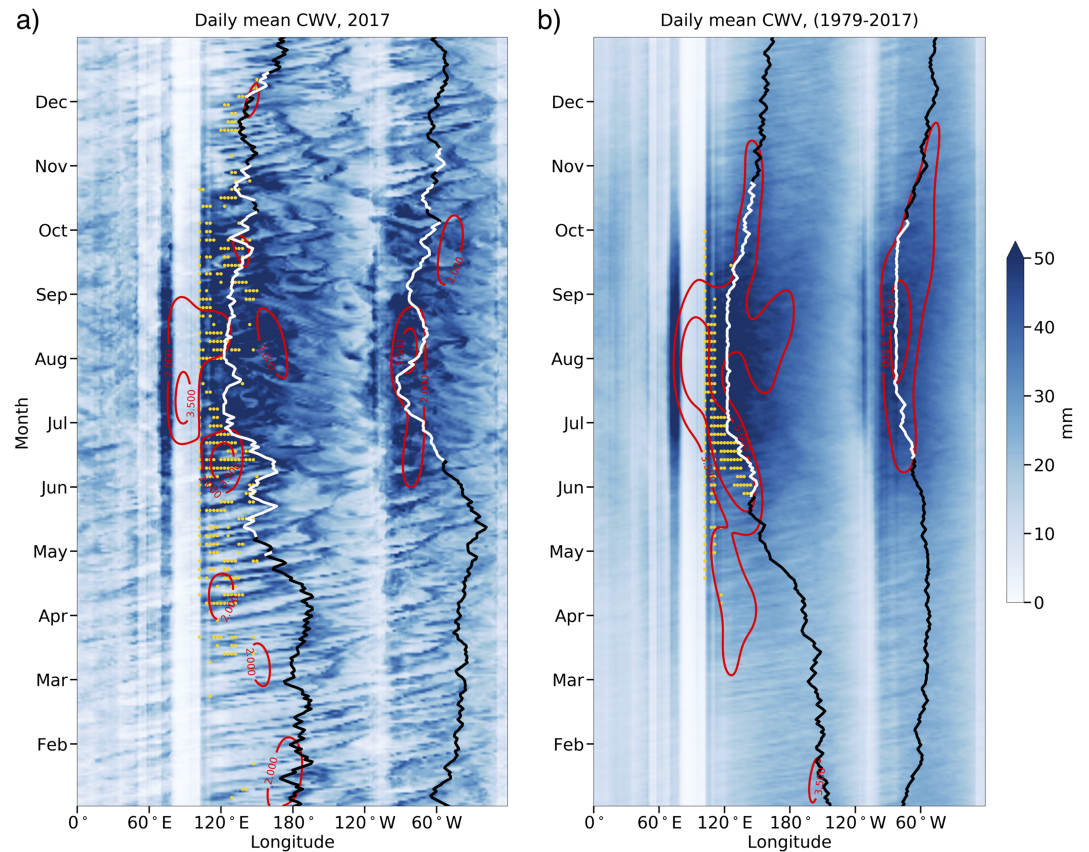
Figure 2. (a) Hovmöller diagram of column water vapor (CWV; 2017) at 30° N with the addition of quasi-stationary part of atmospheric rivers pathways marked by white curves (with the amount of 7-day moving averaged CWV above 40 mm) and black curve (below 40 mm). Yellow stippling indicates areas that satisfy the monsoon index, and the red contours are smoothed precipitation (mm/day). (b) Same as (a) but for 39-year (1979–2017) climatological mean.
