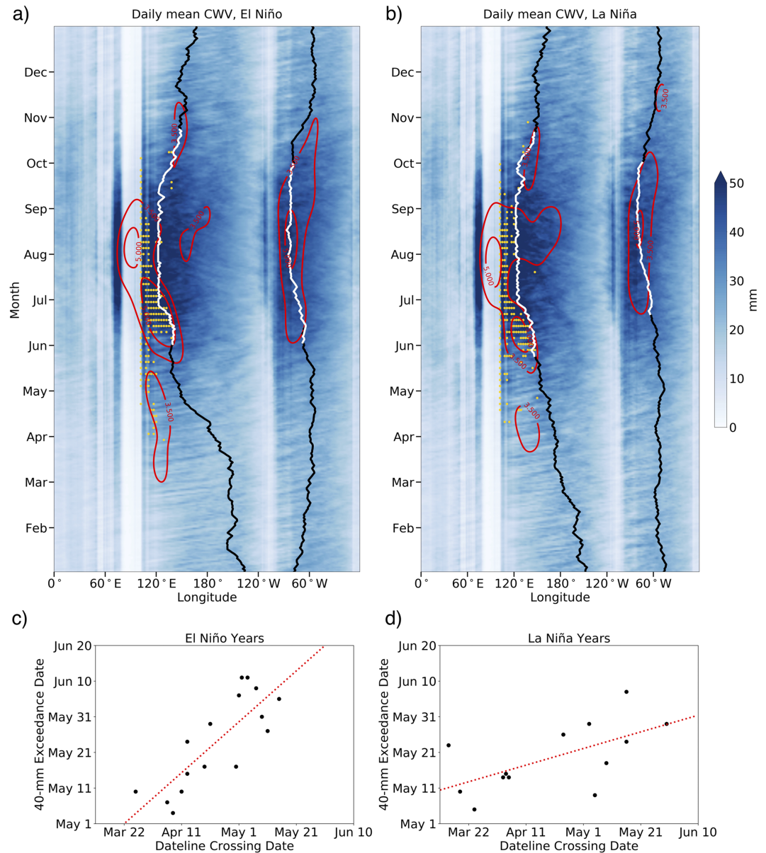
Figure 3. (a) Same as Figure 2 but for El Niño (decaying El Niño). (b) Same as (a) but for La Niña (decaying La Niña). Enclosed quasi-stationary part of atmospheric rivers pathways of El Niño/La Niña are not required unlike 5- and 39-year climatology (see Appendix A). (c) The scatter plot of 40-mm exceedance date of the quasi-stationary part of atmospheric river (our monsoon onset proxy) without an outlier in 1992, and the date when the zonal average of 30° N column water vapor (CWV) on 180–120° W is greater than 120° E–180° W (dateline crossing) during El Niño with the slope 0.71, intercept 63 days, correlation coefficient 0.81, and p value 0.0002 by linear regression analysis. El Niño years here are selected when Niño 3.4 index in May is above 0.25. (d) Same as (c) but for La Niña with the slope 0.23, intercept 113 days, correlation coefficient 0.61, and p value 0.026. La Niña years here are selected when Niño 3.4 index in May is below -0.25 .
