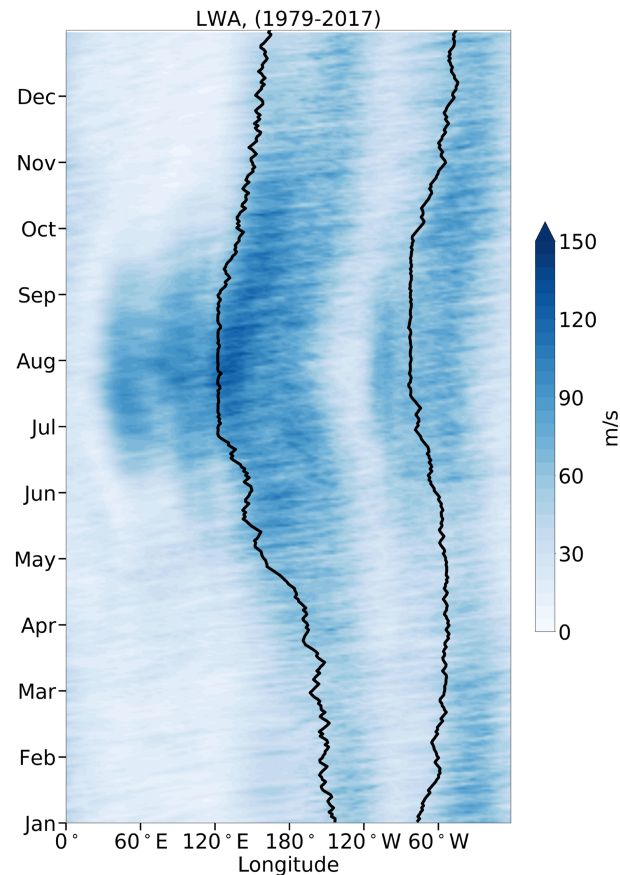
Figure 4. The Hovmöller diagram of daily mean climatology local wave activity (LWA), a measure of the nonlinearity of waves, at 30° N with the addition of quasi-stationary part of atmospheric rivers pathways (black curves).
