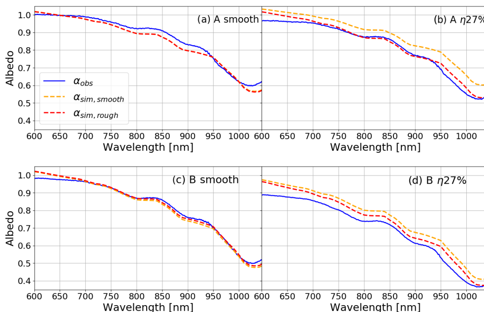
Figure 5. Measured spectral albedo \alpha_{obs} (blue solid lines), and spectral albedo simulated with RSRT by considering the surface as smooth ( \alpha_{sim,smooth} ; orange dashed lines) and by considering surface roughness ( \alpha_{sim,rough} ; red dashed lines) for (a) A smooth, (b) A \eta 27\% , (c) B smooth and (d) B \eta 27\% .
