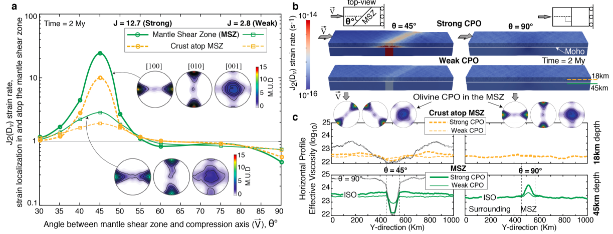
Figure 3: (a) Strain localization at steady-state ( \sim 2 My) as a function of the orientation of the fossil mantle shear zone relative to the imposed shortening ( \theta , loading-geometry). The strain localization is quantified by the ratio between the average of the 2 nd invariant of the strain rate J_2(D_v) in the fossil mantle shear zone (MSZ: green full lines) or in the crust right above it (yellow dashed lines) relatively to the surrounding upper mantle or crust, respectively. Simulations were performed for either strong ( J = 12.7 , thick lines) or weak olivine CPO ( J = 2.8 , thin lines) in the fossil mantle shear zone. (b) Strain rate field at steady-state in simulations with two different orientations of the fossil strike-slip mantle shear zone relative to the imposed shortening ( \theta = 45^\circ or 90^\circ ), in which either the strong or the weak olivine CPO was ascribed to the mantle shear zone. Pole figures illustrate the orientation-relation between the olivine CPO in the fossil mantle shear zone and the imposed shortening. (c) Horizontal effective viscosity profiles at 18 km (middle crust) and 45 km depth (uppermost mantle) for the four simulations shown in (b). Black thin dashed lines in (c) are the mantle and crust effective viscosity profiles for the relation between CPO in the mantle shear zone and surrounding upper mantle that results in the maximum contrast in mechanical behavior (i.e., [100]-axes at 45^\circ and 90^\circ to the compression direction, respectively). Pole figures are contoured at one multiple of a uniform distribution interval.
