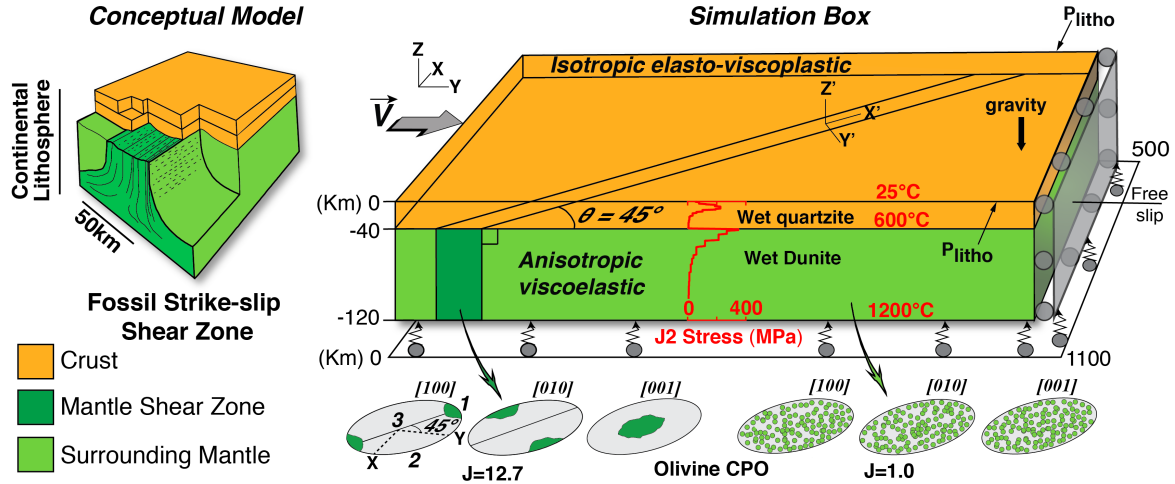
Figure 2: Setup for simulating the compressional deformation of a continental plate containing a 50 km wide fossil strike-slip shear zone in the upper mantle, but a homogeneous crust. The mantle shear zone displays an olivine CPO consistent with seismic anisotropy measurements in lithospheric-scale strike-slip shear zones, characterized by maximum concentrations of olivine [100]- and [010]-axes horizontal, respectively parallel and normal to the shear zone trend, and a vertical alignment of [001]-axes (Vauchez and Nicolas, 1991). The orientation of the mantle shear zone relative to the imposed compression axis ( \theta , loading-geometry) varies between 30^\circ and 90^\circ . In the reference case presented here, the preexisting mantle shear zone is at 45^\circ to the shortening direction ( \theta = 45^\circ ) and has a strong olivine CPO ( J = 12.7 ), whereas the surrounding upper mantle has a random CPO ( J=1.0 ). The external (XYZ) and mantle shear zone (X'Y'Z') reference frames are shown on the top view of the simulation box, and the lithospheric strength profile, the temperature and lateral boundary conditions used in the reference simulation in the lateral view. Average mesh sizes in the crust and mantle are 5 and 10 km, respectively.
