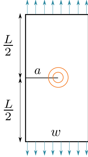
Figure 2: Cracked plate with loading of the reference problem (blue) and of the adjoint problem (orange)
