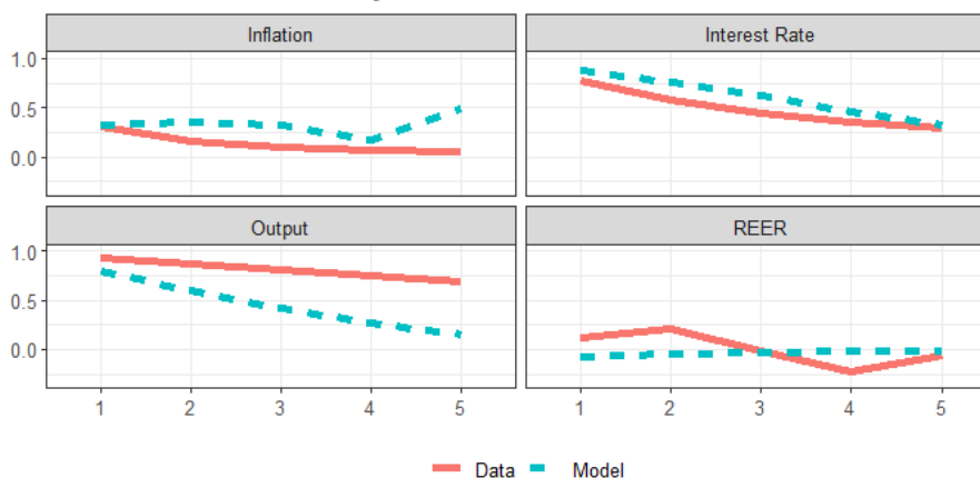
Figure 3: Autocorrelation
