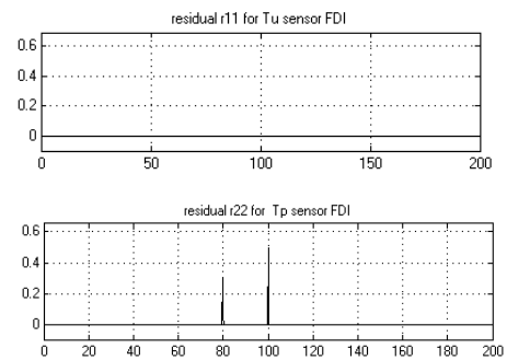
Fig.6 isolation residual in case 1.
