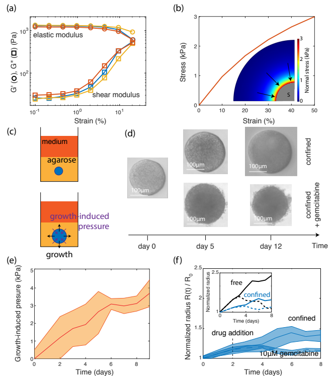
FIG. 2. Effect of gemcitabine on confined growth. a. Measurements of elastic ( G' , \circ ) and shear ( G'' , \square ) moduli of 1% low-melt agarose. Different colors correspond to different forces used to hold the sample. b. Comsol simulation of a spheroid growing in a Neo-Hookean material modeled with parameters extracted from (a). Inset: Heat map of normal stress onto a spheroid (grey, S). c. Schematic of agarose-confined spheroid. d. Representative pictures of a confined spheroid and one treated with gemcitabine. e. Growth-induced pressure of spheroids in 1% low-melt agarose as a function of time. Median values normalized to time 0 \pm \text{SD} over N \geq 20 spheroids. f. Growth quantification of confined spheroids and treated ones with drug. Inset: Median curves for free (black) and confined (blue) spheroids, dashed lines correspond to gemcitabine treatment. Median \pm SD over N \geq 20 spheroids. Time 0 correspond to agarose confinement.
