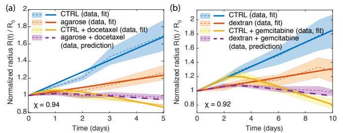
FIG. 4. Prediction of the model for (a) confined spheroids exposed to docetaxel ( \chi = 0.94 ) and (b) osmotically compressed spheroids exposed to gemcitabine ( \chi = 0.92 ). In both cases, median values normalized to the time of drug addition \pm SD over N \geq 10 spheroids for docetaxel and \geq 30 spheroids for dextran. Drug was added at time 0 for (a) and at time 2 for (b).
