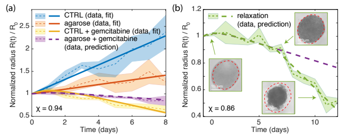
FIG. 3. Prediction of the model on confined data. a. Model plotted on confined spheroids exposed to gemcitabine (large dashed purple). Prediction score \chi = 0.94 . b. At drug addition, R(t=0) \geq R(t=-2) , while at about day 7, the radius decreases due to drug treatment to a value R(t=7) \sim R(t=-2) and become unconfined: subsequent decrease happens without mechanical stress. The model (large dashed green) captures this effect, switching from rate of confined cells (large dashed purple), to rate of unconfined cells. \chi = 0.86 . In both cases, median values normalized to the time of drug addition \pm SD over N \geq 20 spheroids. Time 0 correspond to drug treatment.
