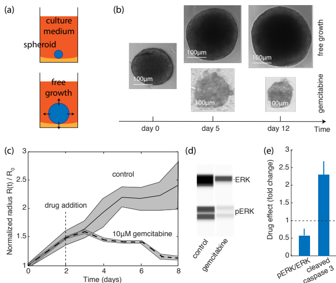
FIG. 1. Effect of gemcitabine on free growth. a. Schematic of free growing spheroid. b. Representative pictures of growing spheroids and one treated with gemcitabine after two days. c. Growth quantification over time. Median values normalized to time 0 \pm \text{SD} over N \geq 30 spheroids. d. Example of capillary western blot after 5 days under drug. e. Analysis of capillary western blots. The data under gemcitabine treatment are normalized to the control. Mean \pm SEM over N \geq 3 replicates. Data were pooled together. The quantity was renormalized by total volume of spheroids.
