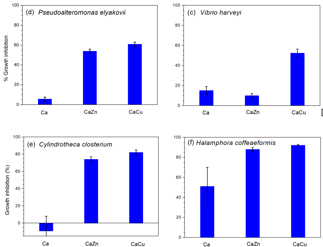
Figure 5. Evaluation of growth inhibition of four bacteria: Halomonas aquamarina (a), Vibrio aesturianus (b), Vibrio harveyi (c), Pseudoalteromonas elyakovii (d) and two microalgae strains: Cylindrotheca closterium (e) and Halomphora coffeaformis (f).
