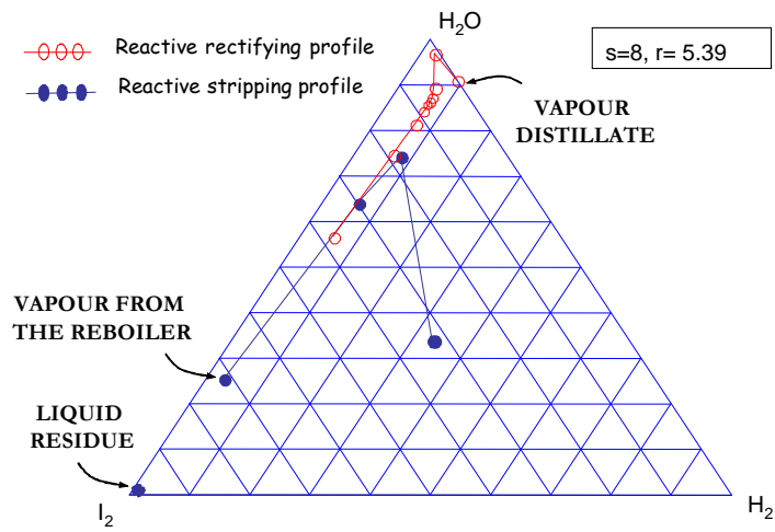
Figure 13. Vapour reactive profiles in the reactive distillation column of a ternary HI-I 2 -H 2 O mixture for s=8 and r=5.39
