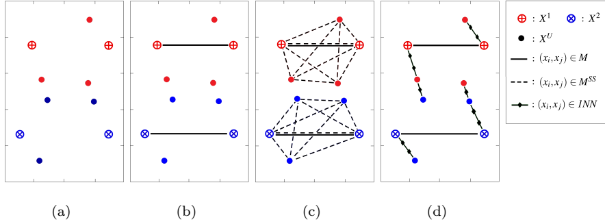
Figure 1: Must-link pairs in a semi-supervised learning context. (a) Set of unlabeled data samples (displayed with color of class labels for a better interpretation of results) and two prototype sets X^1 and X^2 . (b) Set M . (c) Set M^{SS} . (d) Set 1NN Links corresponding to similarity matrices W^{KNN1} , W^{KNN2} , W^{KNN3} and W^{KNN4} .
