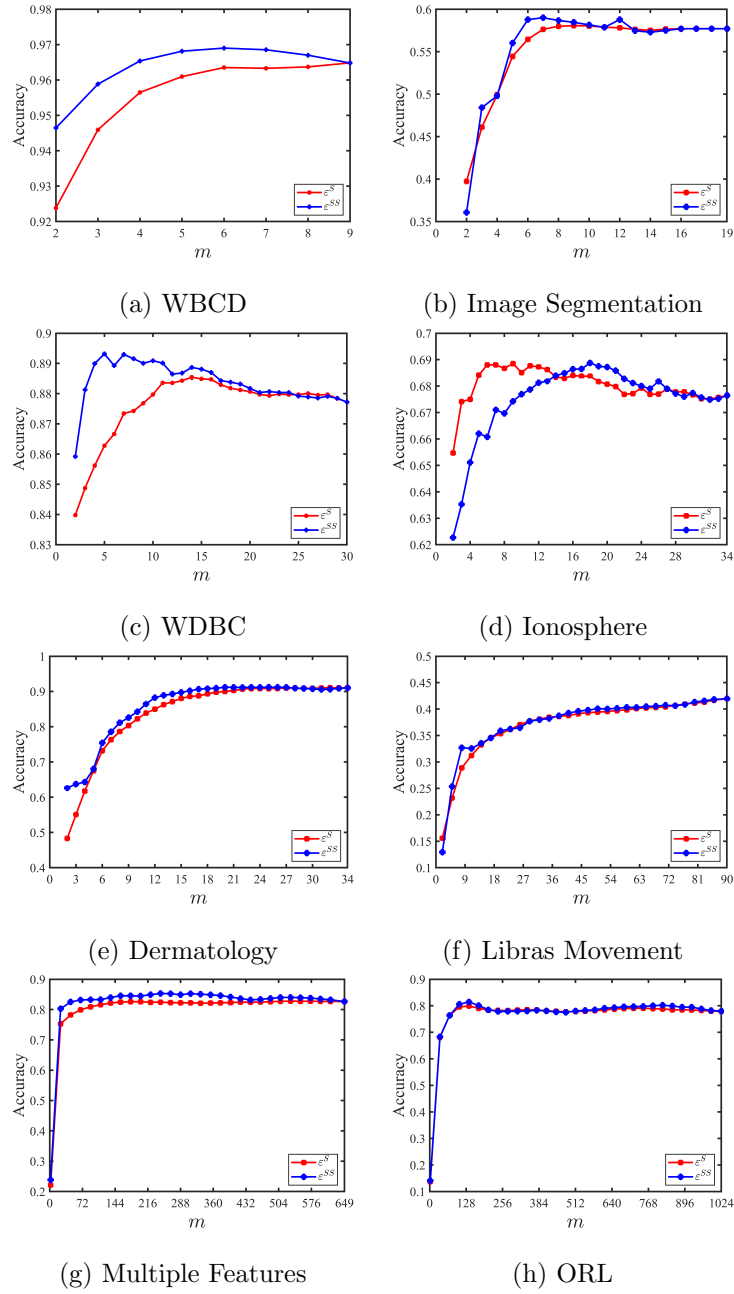
Figure 10: Comparison of accuracy rates obtained by \epsilon^{SS} and \epsilon^S scores for eight benchmark databases using nearest neighbor classifier
