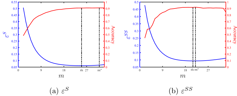
Figure 9: Accuracy-scores \varepsilon^S and \varepsilon^{SS} versus number of selected features for the Dermatology database
