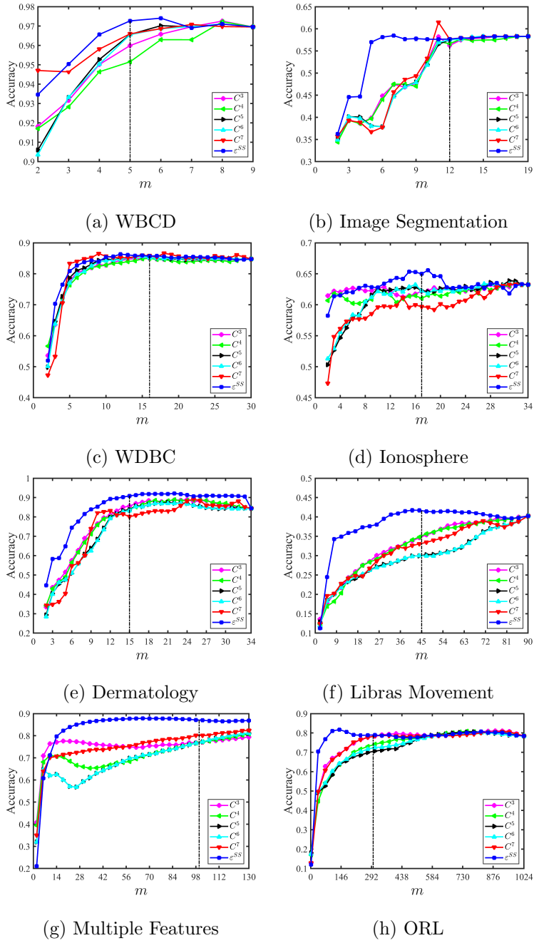
Figure 6: Accuracy versus number of selected features m by the semi-supervised constraint scores for eight benchmark databases
