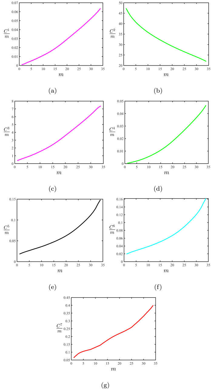
Figure 2: State-of-the-art constraint scores with respect to the number of selected features m for the Dermatology database: (a) \frac{C^1}{m} , (b) \frac{C^2}{m} , (c) \frac{C^3}{m} , (d) \frac{C^4}{m} , (e) \frac{C^5}{m} , (f) \frac{C^6}{m} , (g) \frac{C^7}{m}
