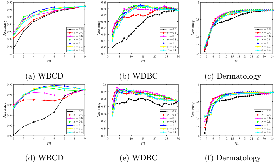
Figure 8: Influence of the scaling parameter \sigma versus number of selected features m by the proposed constraint scores \varepsilon^S and \varepsilon^{SS} . Top row: results obtained by using \varepsilon^S . Bottom row: results obtained by using \varepsilon^{SS}
