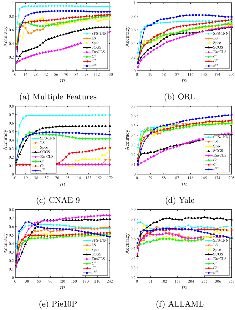
Figure 7: Accuracy versus number of selected features m by semi-supervised and unsupervised feature selection methods on six high dimensionality databases
