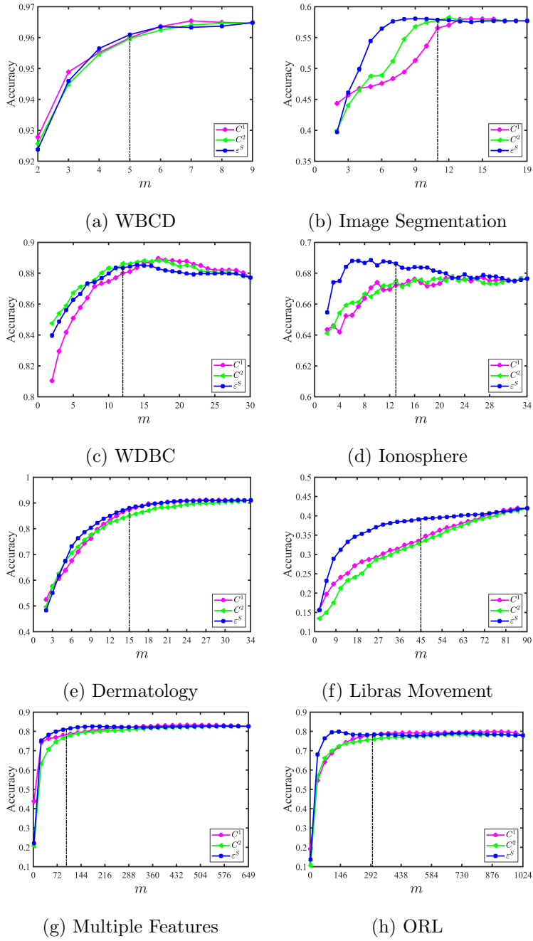
Figure 4: Accuracy versus number of selected features m by the supervised constraint scores on eight six benchmark databases
