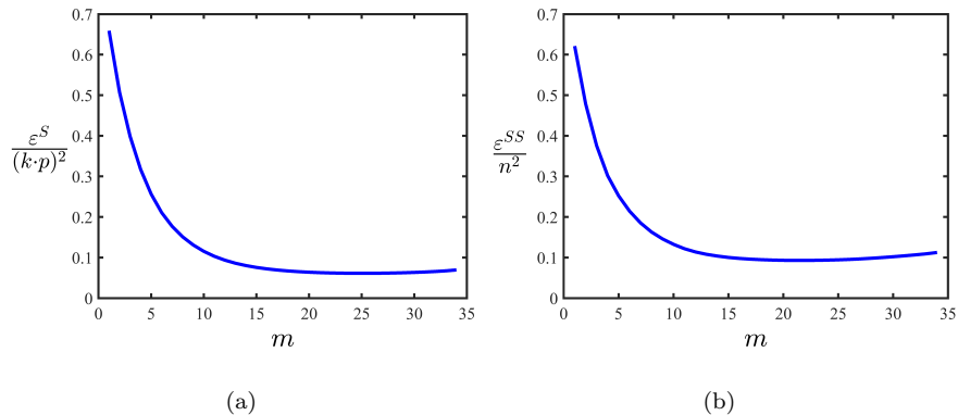
Figure 3: Proposed constraint scores with respect to the number of selected features m for the Dermatology database: (a) \frac{\varepsilon^S}{(k \cdot p)^2} and (b) \frac{\varepsilon^{SS}}{n^2}
