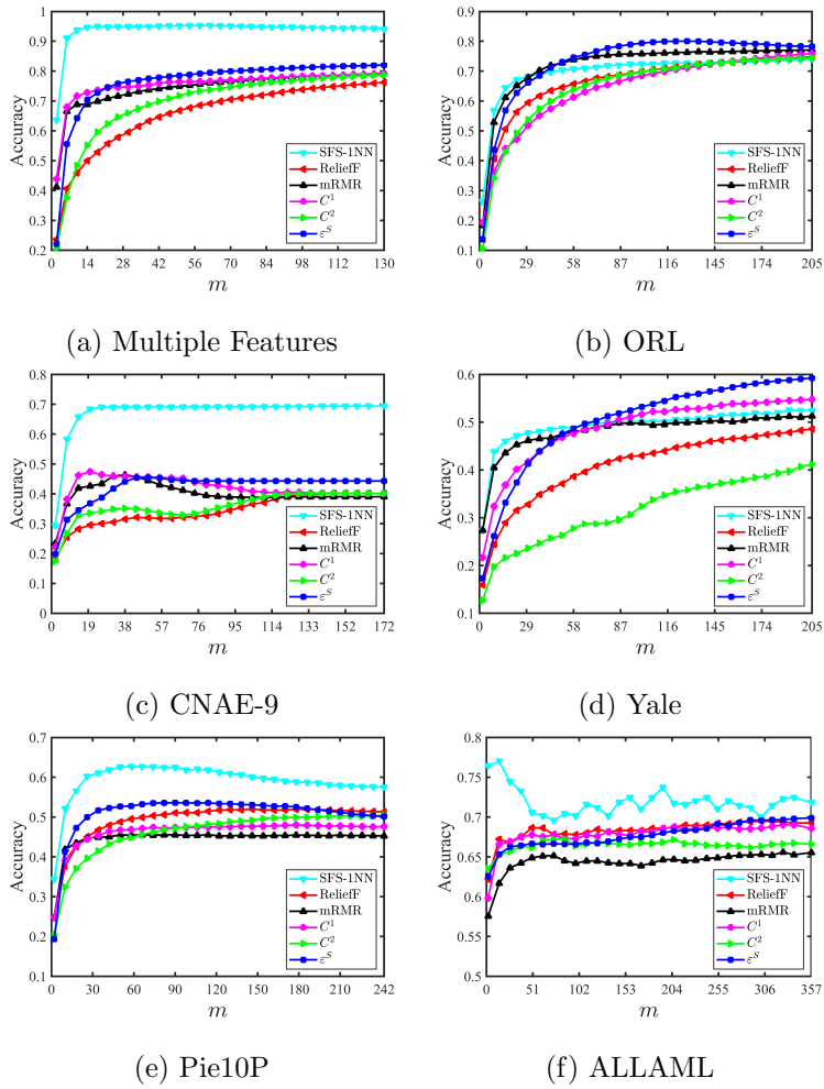
Figure 5: Accuracy versus number of selected features m by supervised feature selection methods on six high dimensionality databases
