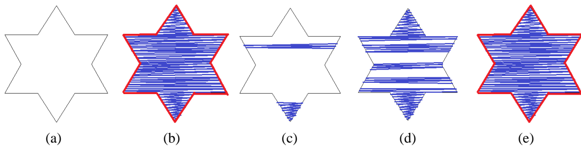
Figure 6. Random segmentation of area-filling motions to achieve uniform heat distribution: (a) Contour; (b) Area-filling path; (c), (d), (e) random writing of the segments.
