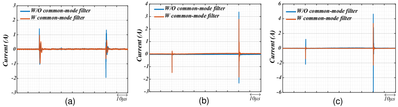
Fig. 11: Experimental results of measured common-mode currents in 1200V, 150A double pulse test (a) ICML (b) ICMH (b) Input- ICM.
