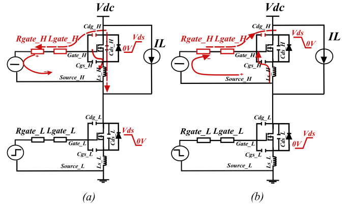
Fig. 3: Gate voltage perturbation mechanism (a) Positive perturbation during turn-on (b) Negative perturbation during turn-off.
