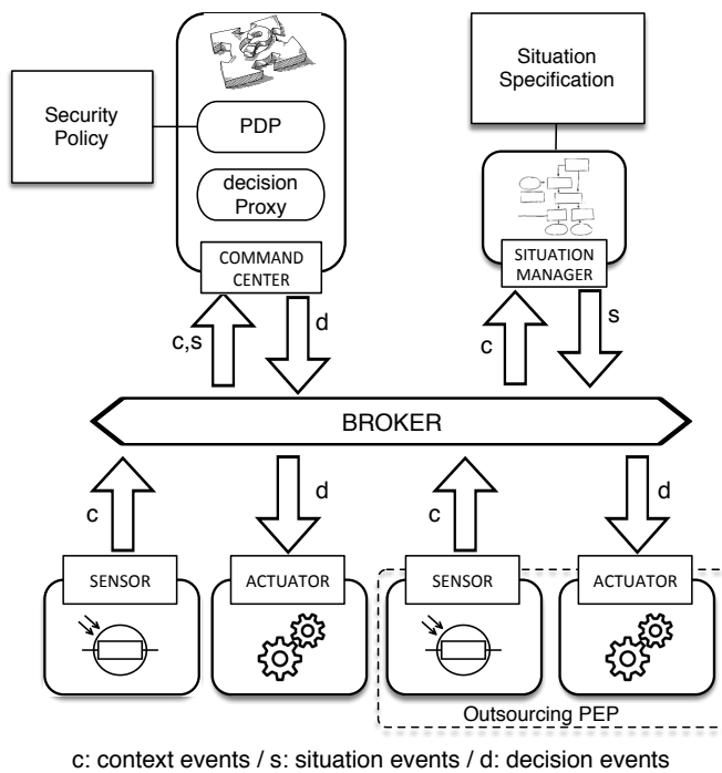
Figure 4. The dynSMAUG deployment architecture
