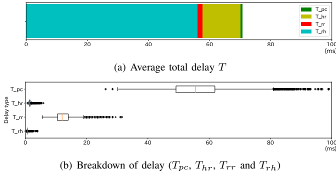
Fig. 5. Total delay and the breakdown
