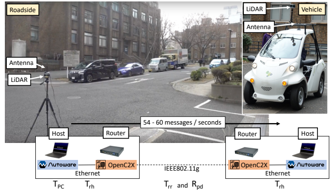
Fig. 4. Experimental setup
