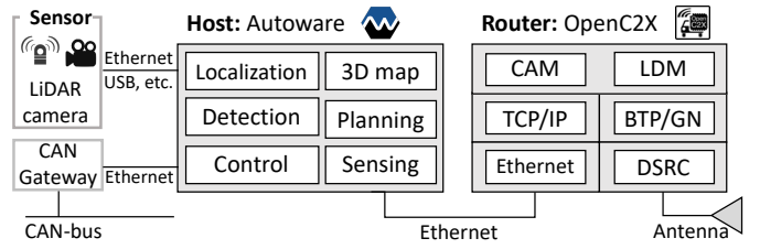
Fig. 1. System model to integrate Autoware and OpenC2X
