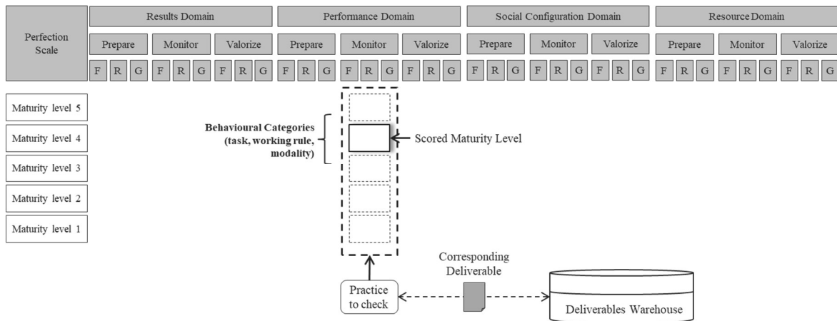
Fig.2. Example of the Evaluation structure
