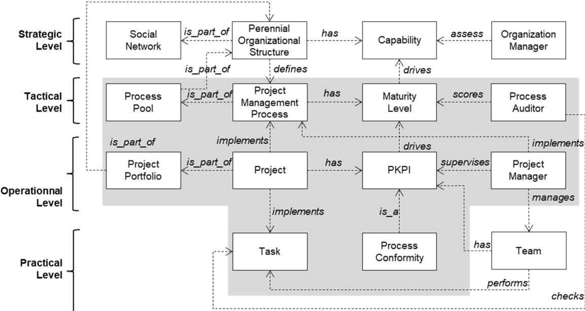
Fig.1. Maturity Model Conceptual Framework.
