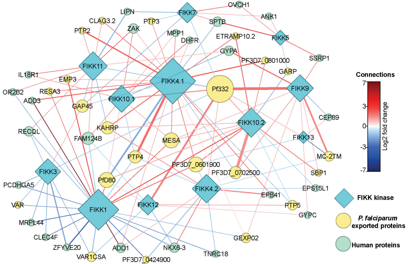
Figure 4. FIKK kinases are part of a complex network and act in synergy Network analysis of human RBC proteins (green) and P. falciparum exported proteins (yellow) which are significantly changing upon deletion of the FIKK kinases (blue). The thickness of the connecting lines represents the number of phosphosites significantly changing on each protein due to deletion of each kinase, while lines are coloured according to the average log 2 fold change of all the significantly-changing phosphosites. Symbol size represents the number of connections to each protein.
