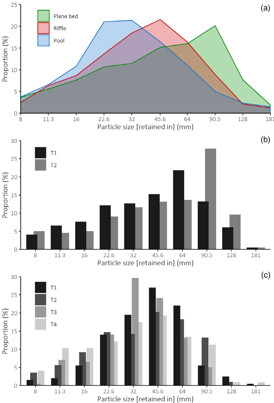
FIGURE 3 Histograms of GSD per morphological unit. (a) Average distributions for the entire study period. Changes on GSD fractions for the (b) plane bed and (c) riffle morphologies. Only GSD at sampling occasions that were found to be statistically different ( \chi^2 ) are shown [Colour figure can be viewed at wileyonlinelibrary.com ]
