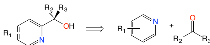
Scheme 1. General strategy for the synthesis of \alpha -substituted pyridinemethanols (carbinols).
