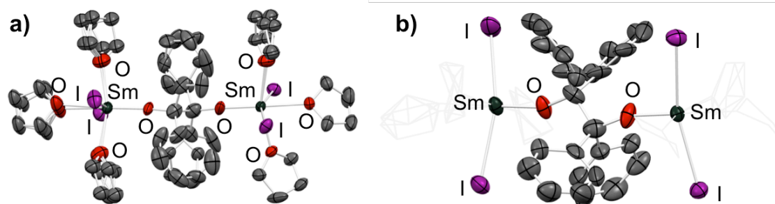
Figure 1. ORTEP of 1 . Thermal ellipsoids are at 50% level. 1a and 1b are two different views. In 1b, the thf are shown in light grey wireframes.
