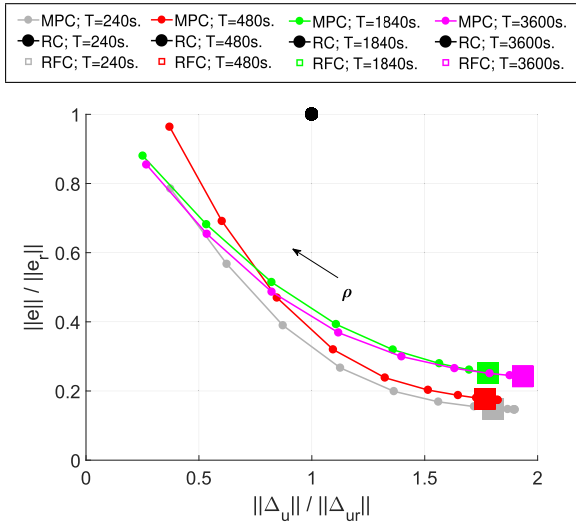
(a) Relative error norm of energy versus relative management effort.
