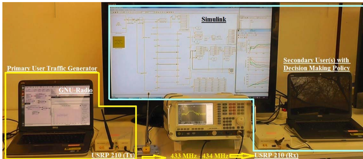
Figure 1. Left hand side (laptop with GNU Radio + USRP) is generating primary user traffic on 8 channels (Tx). Right hand side (laptop with Simulink + USRP) is a secondary user employing energy detector for channel sensing and online learning algorithm based learning policies (Rx). A spectrum analyzer monitors the RF signals.
