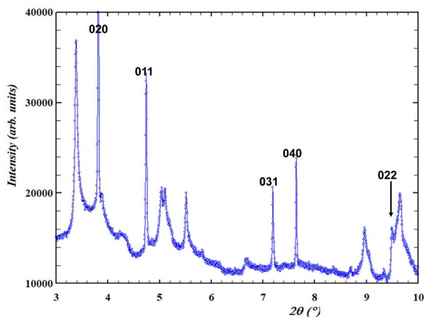
Figure 3. Low-angle region of the synchrotron PXRD pattern for the Cap Garonne specimen. The sharp reflections all index as (0kl) based on cell parameters b = 17.7 and c = 7.8 Å. The first reflection is (200) where a = 19.9 Å.
