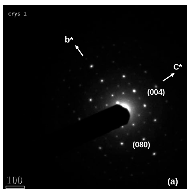
Figure 4. Electron diffraction (0kl) reciprocal lattice section for the Cap Garonne specimen. (b) Image of flat lath crystal used to obtain the ED pattern. Museums Victoria specimen M55455.
