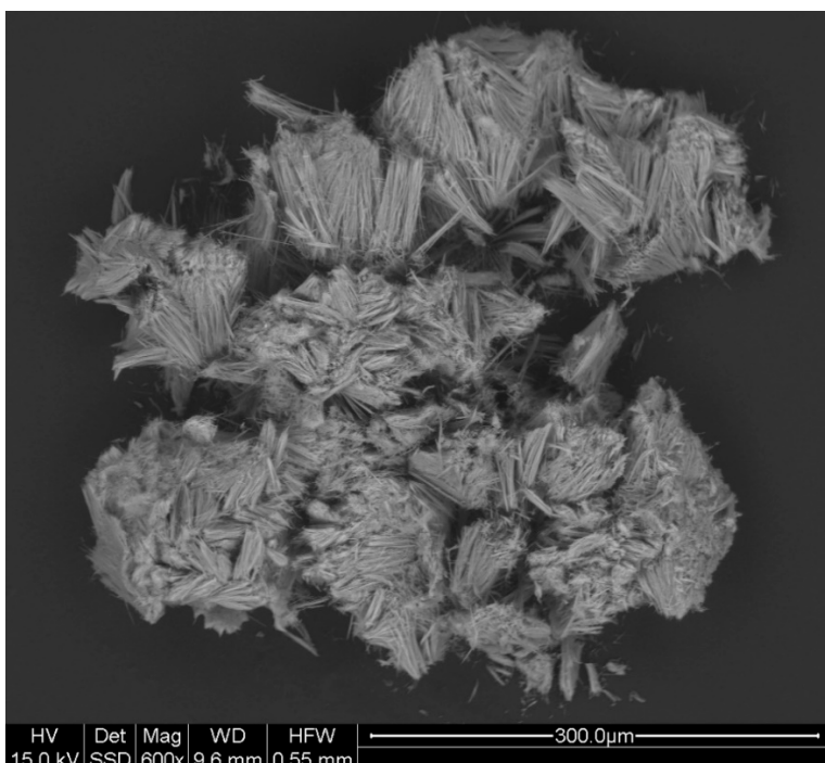
Figure 2. SEM back-scattered electron image of clumps of fibrous bulachite crystals from Cap Garonne. Museums Victoria specimen M55455.
