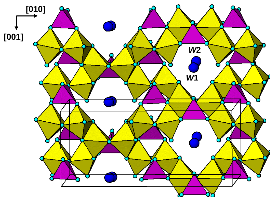
Figure 10. Projection approximately along [100] of the structure of bulachite, showing spirals along [001] of edge-shared Al-centred octahedra (yellow) and corner-connected AsO 4 tetrahedra (mauve).
