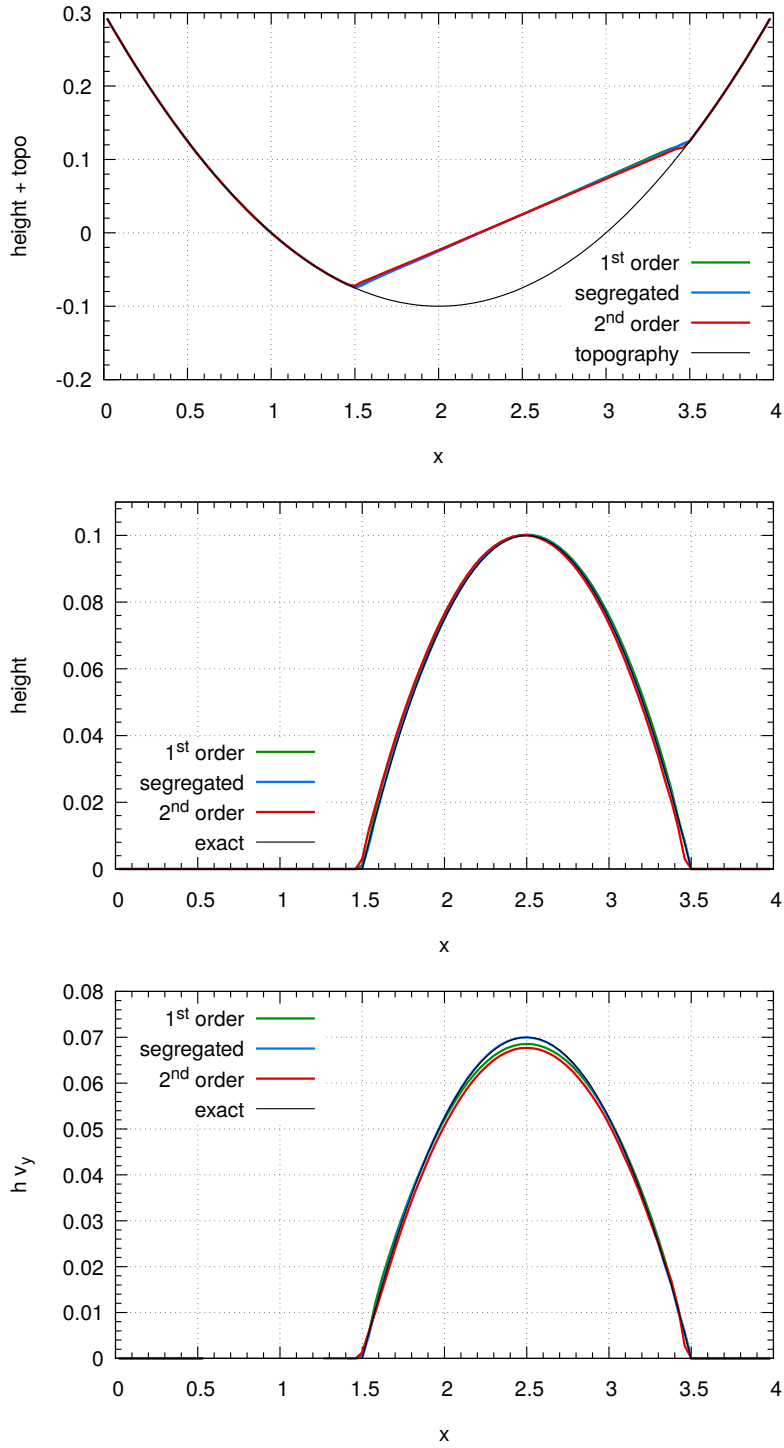
FIGURE 9. Circular motion of a drop over a paraboloid-shaped topography. Sum of the height and the topography, height alone and second component of the momentum along the y = L/2 line at t = 6\pi .
