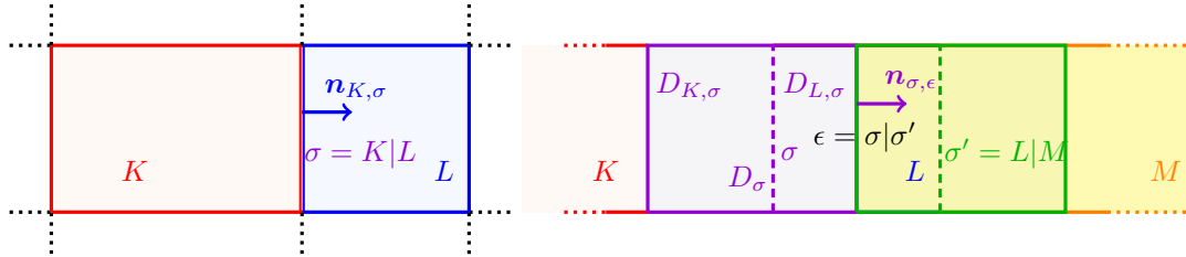
FIGURE 1. Notations for the primal and dual meshes (in two space dimensions, for the first component of the velocity).
