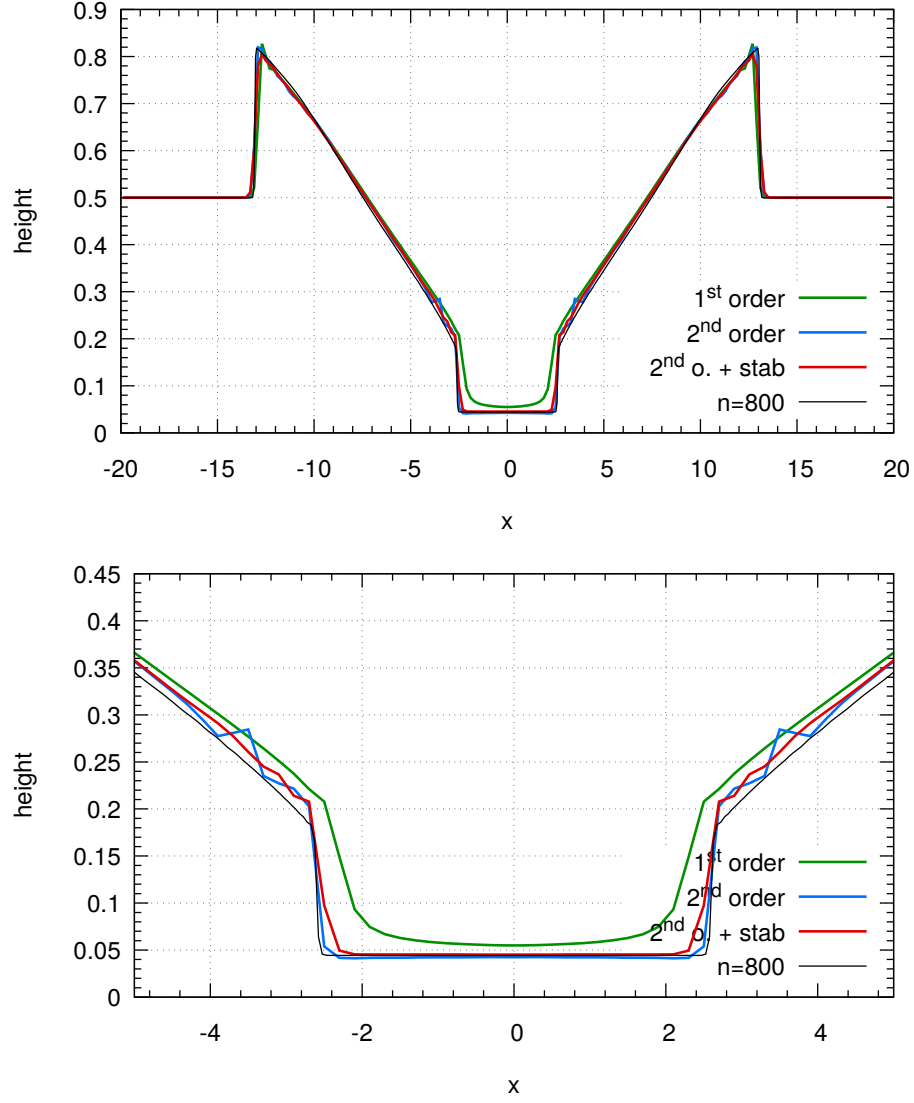
FIGURE 7. Circular dam-break problem. Height obtained at t = 3T/5 with the first-order scheme and the second-order scheme with and without stabilization, with a 200 \times 200 mesh.
