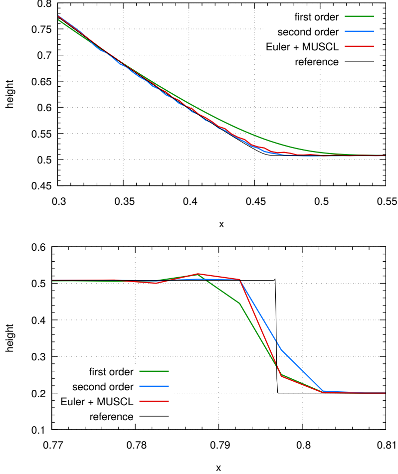
FIGURE 4. Riemann problem. Details of the flow height.
