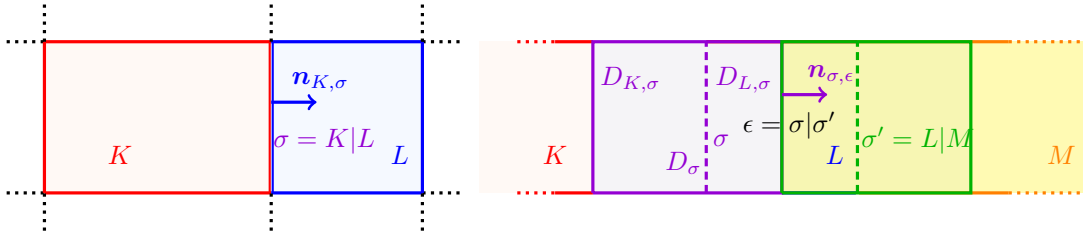
FIGURE 1. Notations for the prima and dual meshes (in two space dimensions, for the first component of the velocity).
