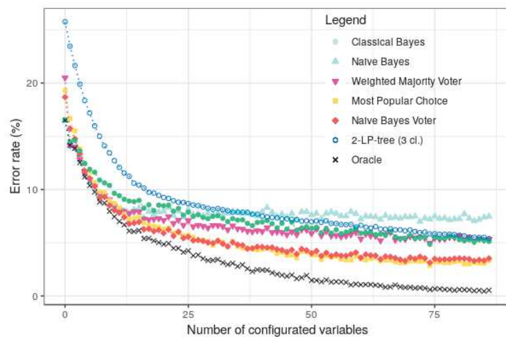
Figure 5: Average error rate on datasets Renault-44 (top) Renault-48 (middle) and Renault-87 (bottom)
