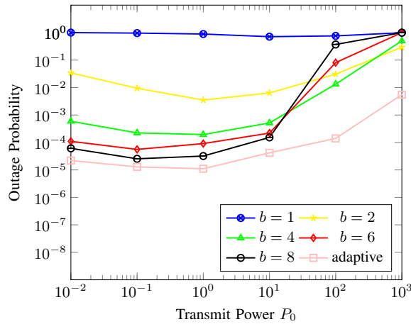
Fig. 2: Outage probability for coordinated-fair approach with different values of b . Here, \lambda = 1 , \lambda_e = 0.1 , d_{\max} = 5 , \lambda_r = 1 .
