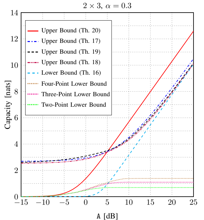
Fig. 10: Bounds on capacity of the same 2 \times 3 MIMO channel as discussed in Figure 9, and average-to-peak power ratio \alpha = 0.3 .
