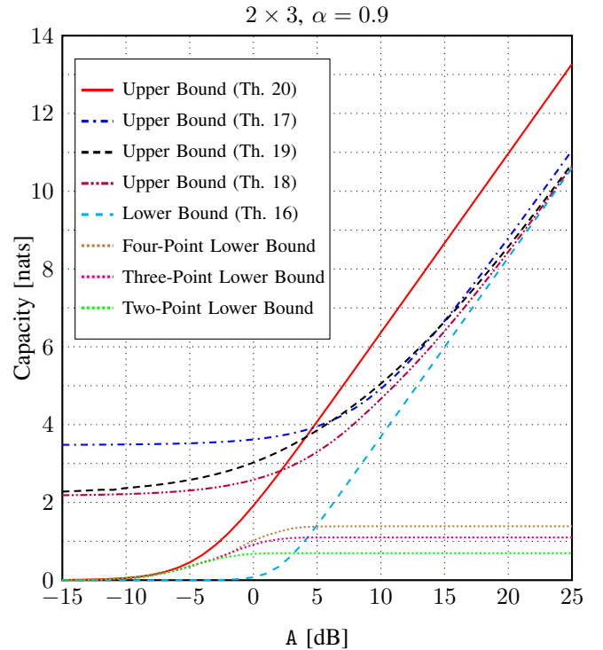
Fig. 9: Bounds on capacity of 2 \times 3 MIMO channel with channel matrix \mathbf{H} = [1, 1.5, 3; 2, 2, 1] , and average-to-peak power ratio \alpha = 0.9 . Note that the threshold of the channel is \alpha_{\text{th}} = 1.4762 .
