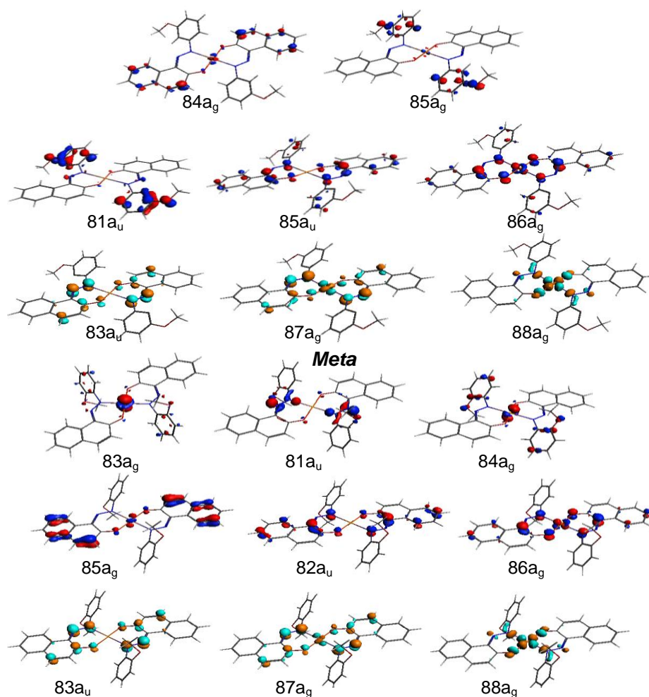
Figure 7. MO plots of the crucial orbitals for (I) (top) and (II) (bottom) isomers. For both complexes (I) and (II), the HOMO and LUMO correspond to 86a g and 83a u MOs, respectively.
