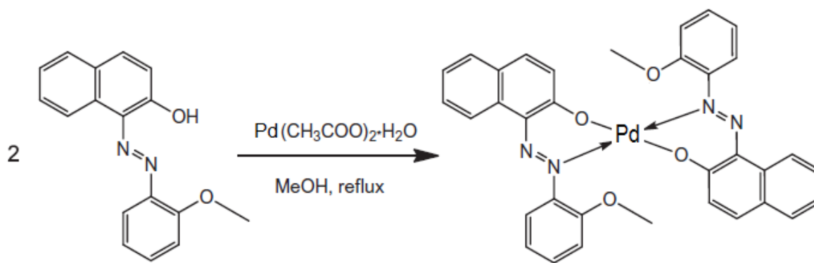
Scheme 1. Reaction route for the Pd(II) complex(I).
