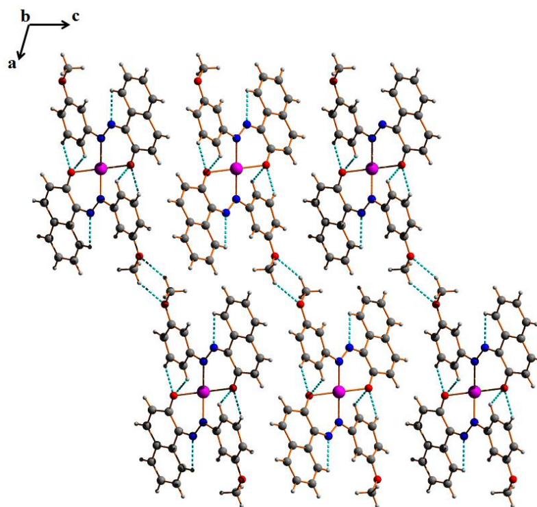
Figure 4. A partial view along the b axis of the crystal packing of the title complex (II), showing the C–H...N and C–H...O interactions which are displayed as dashed lines (see Table 3).
