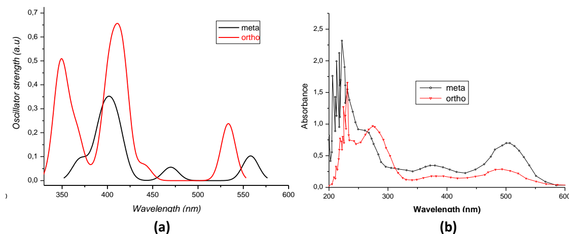
Figure 8. TD-DFT simulated (a) and experimental (b) UV-Vis spectra for complexes (I) and (II) in \text{CH}_2\text{Cl}_2 .
