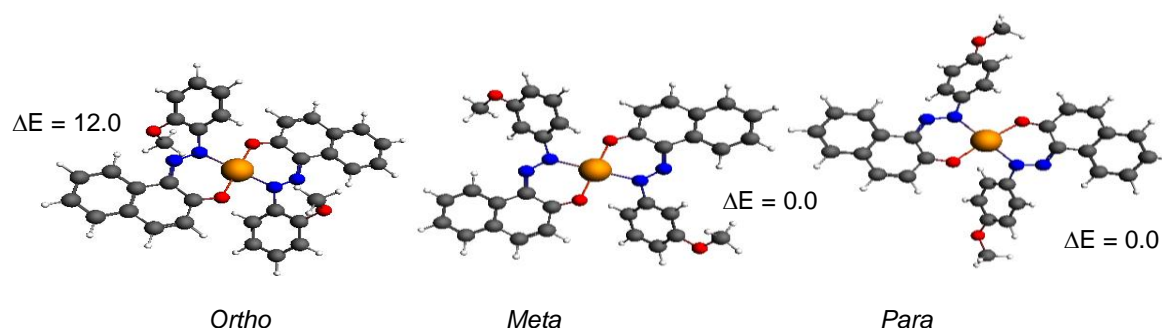
Figure 6. Optimized structures obtained for complexes (I), (II) and (III) in their singlet ground state. Relative energies between isomers \Delta E are given in kcal/mol.
