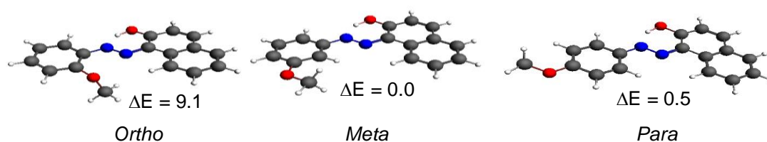
Figure 5. Optimized structures obtained for the free ligand precursor isomers. Relative energies \Delta E are given in kcal/mol.
