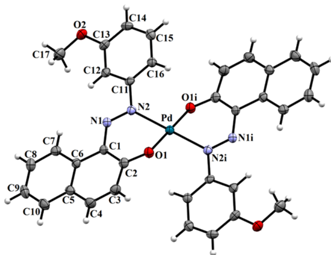
Figure 2. The molecular structure of compound (II), with atom labelling and 50% probability displacement ellipsoids. The unlabelled atoms are related to the labeled atoms by the symmetry operation (-x+2, -y, -z+2) .
