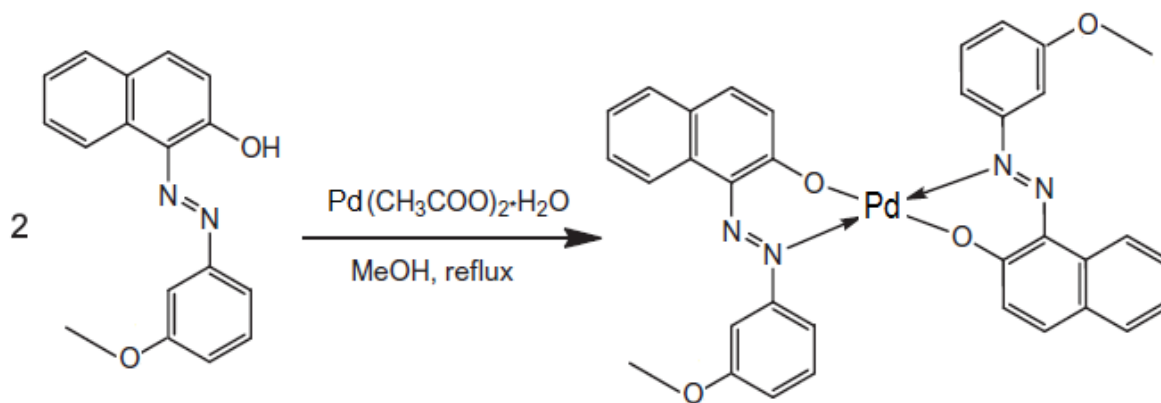
Scheme 2. Reaction route for the Pd(II) complex (II).
