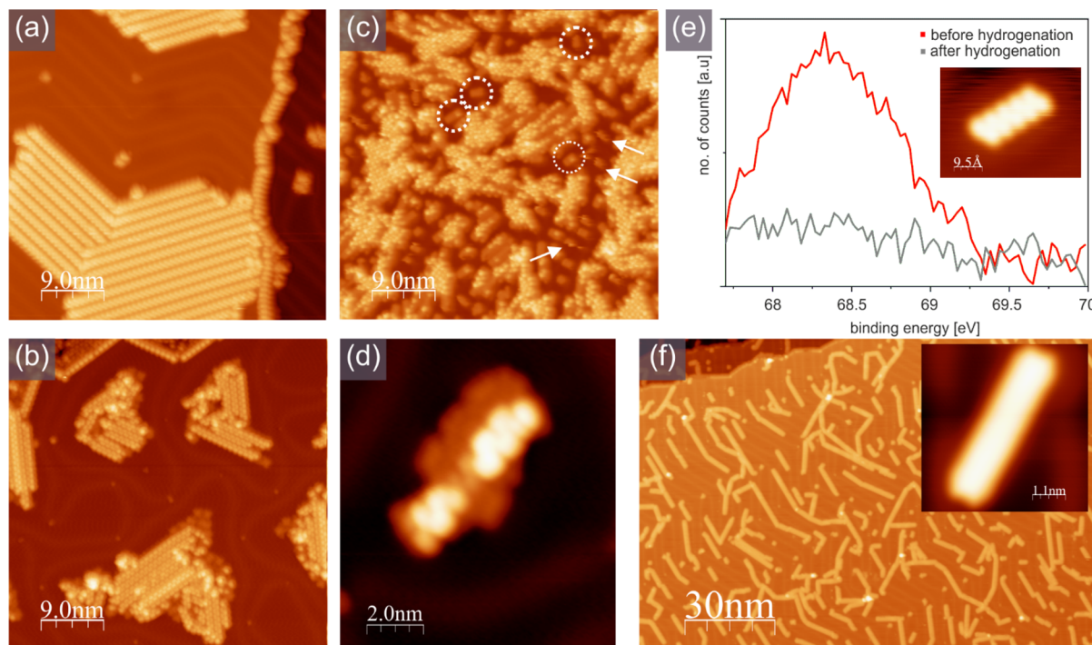
Figure 2. Hydrogen treatment of DBBA precursors: (a) STM image of self-assembled DBBA molecules; (b) DBBA polymers with surrounding Br atoms obtained after annealing at 180 °C; (c) STM image of the sample after atomic hydrogen treatment at 100 °C—the flexible DBBA precursors are found within islands, white dashed circles mark exemplary isolated polymers (magnified image is shown as inset in (e)); white arrows highlight the mobile DBBA polymers; (d) high-resolution STM image of the small island comprised of DBBA polymers after atomic hydrogen treatment at 100 °C—the image clearly shows that the assembly is not planar and contains polymers placed on top of the first layer polymers; (e) XPS data obtained for Br 3d resonance before (red) and after (gray) application of atomic hydrogen flux at 100 °C, disappearance of the resonance resembles effective removal of Br by atomic hydrogen flux (the inset shows high resolution STM image of a single DBBA polymer (0.5 V, 25 pA)); (f) large-scale STM image of 5-AGNRs generated by annealing at 350 °C the sample with DBBA polymers after application of the atomic hydrogen treatment. Scan parameters: -1 V, 50 pA (a, b, f), -1 V, 15 pA (c, d, e).
