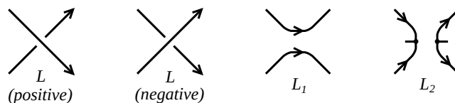
Figure 3.4: Relation in the arrow Kauffman bracket
