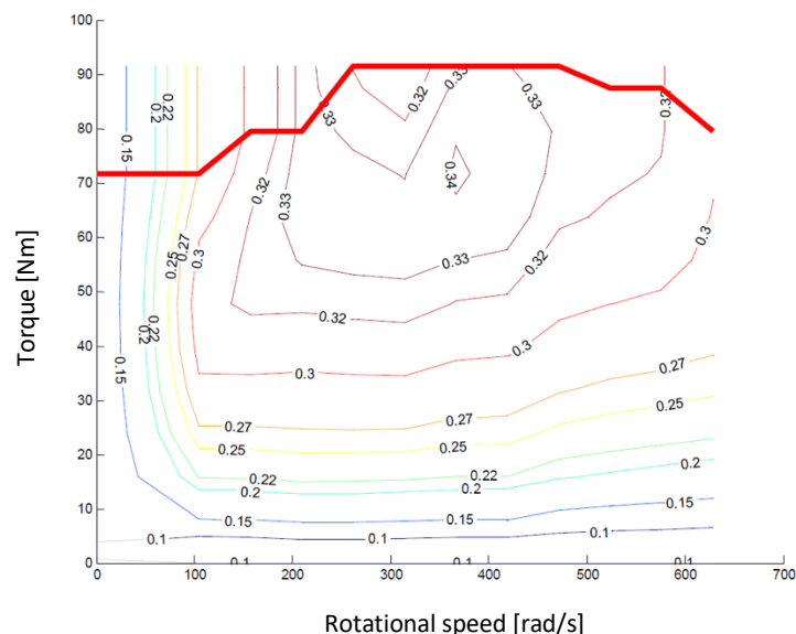
Figure 3-1 Example of efficiency map of a gasoline engine (the red line is the maximum torque curve) [17].
