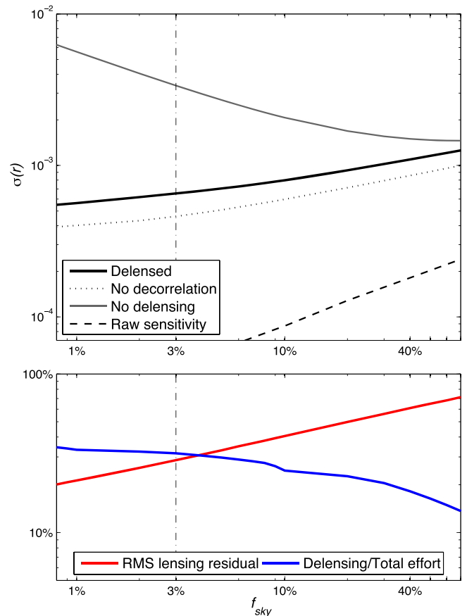
Figure 6. Top: optimized constraints on r as a function of sky fraction, for a fixed effort of 1.2 \times 10^6 150 GHz equivalent detector-years. We include in solid black the case with delensing, allowing for decorrelation of the foregrounds, in solid gray the case without delensing, in dotted gray the case where no decorrelation is allowed in the model (with delensing), and in dashed black the raw sensitivity in the absence of foreground and lensing. Bottom: for the delensed case (with decorrelation), we show the fraction of effort spent on removing the lensing sample variance and the resulting rms lensing residual.
