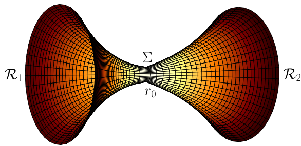
FIG. 3. Embedding diagram for a reflection-asymmetric thin-shell traversable wormhole with parameters M_2 = 1.6M_1 , r_0 = 2.1M_1 , Q_1^2 = 0 , Q_2^2 = 0.98M_2^2 .
