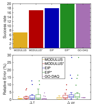
Figure 4: Quantitative assessment using 3 views. Success rate (top), and error distribution (bottom) over 20 triplets sampled from Herz-Jesu-P25 .
