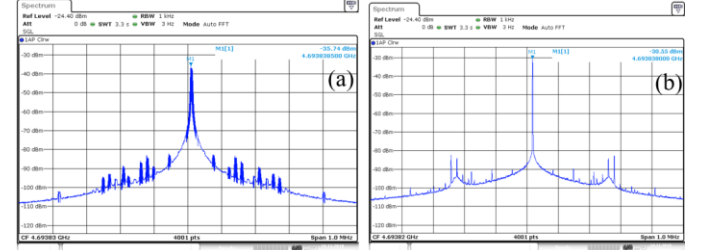
Fig. 6. Output spectrum of the oscillator in respectively (a) free-running mode and (b) locked by injection.
