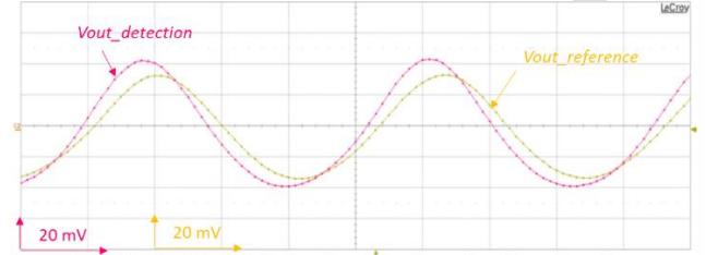
Fig. 10. Output waveforms of the detection system when f_{detFR}=f_{inj} -40 kHz.
