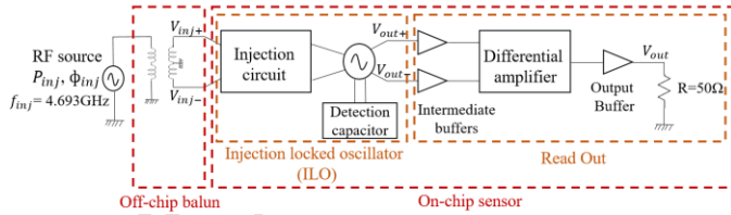
Fig. 2. Detection oscillator schematic implementation.
