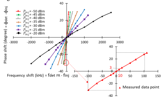
Fig. 7. Single ILO measured phase shift versus the free running frequency variation related to the injection signal one.
