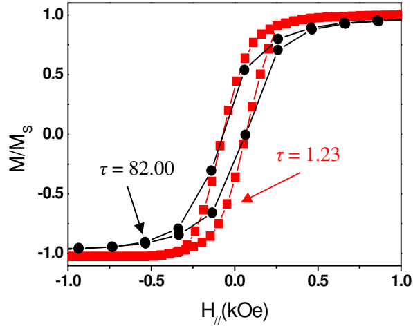
Figure 3. – Normalized magnetization ( M/M_s ) versus applied parallel magnetic field ( H_{\parallel} ): hysteresis loops of the two Ni samples having the extreme geometrical ratio values ( \tau = 1.23 and 82.00 ).
