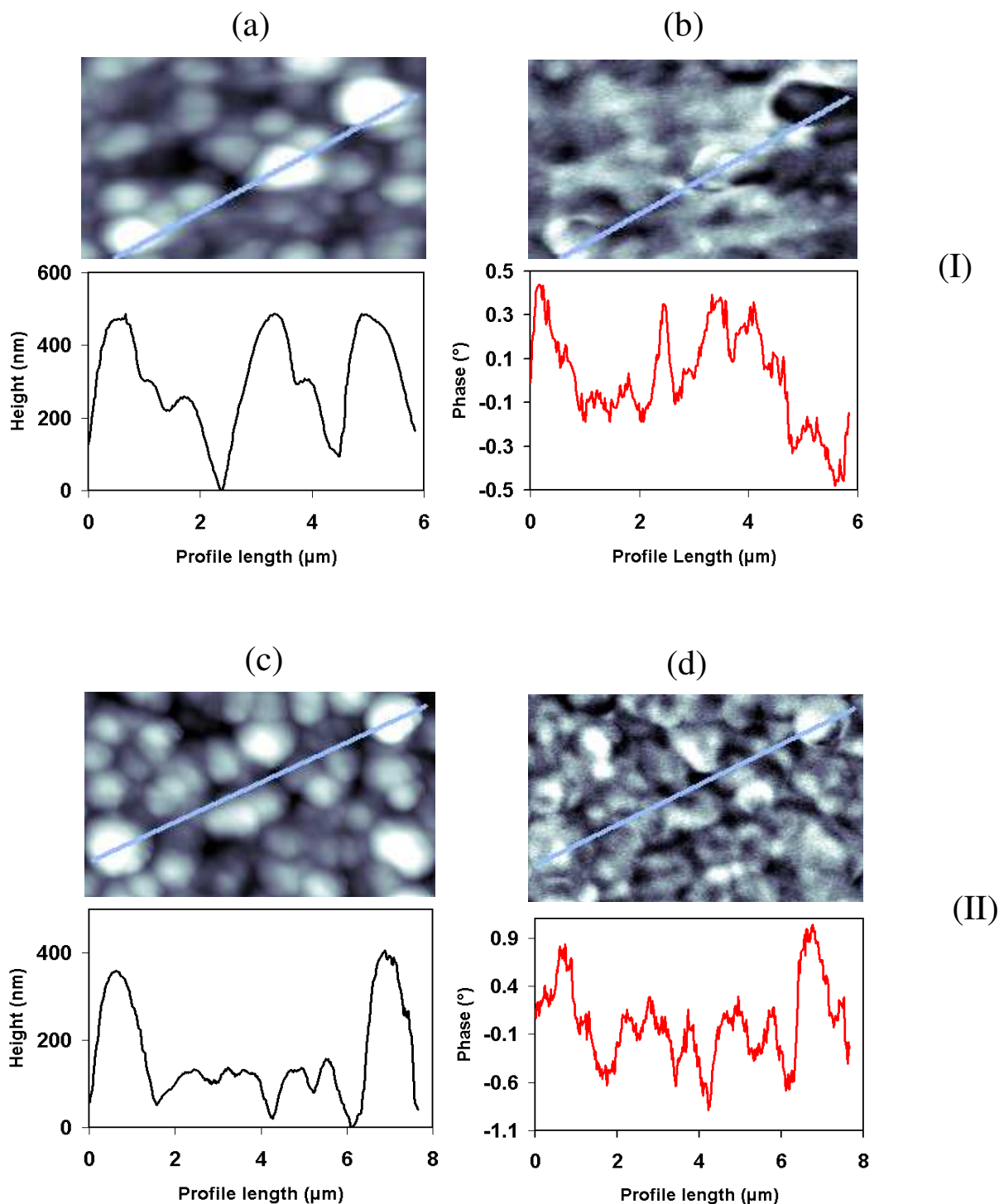
Figure 5. – Local SPM analyses of Ni samples related to the two extreme geometrical ratio values: (I) – (a) topography image and profile; (b) magnetic phase image and profile for the sample labeled \tau = 1.23 . (II) – (c) topography image and profile; (d) magnetic phase image and profile for the sample labeled \tau = 82.00 .
