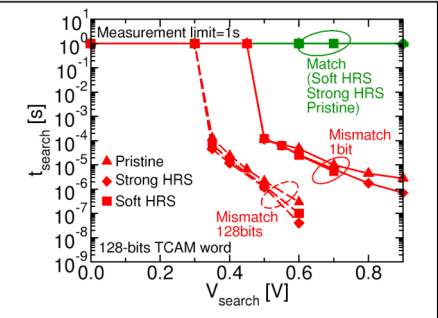
Fig.8: Measured search times at different search voltages, in case of match (green) and mismatch (red).
