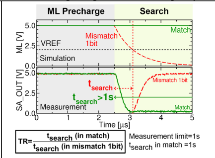
Fig.7: Waveforms of the search operation for a match (green) and mismatch (red). The search time is the time required to discharge the ML to VREF from the pre-charged value (VDD).
