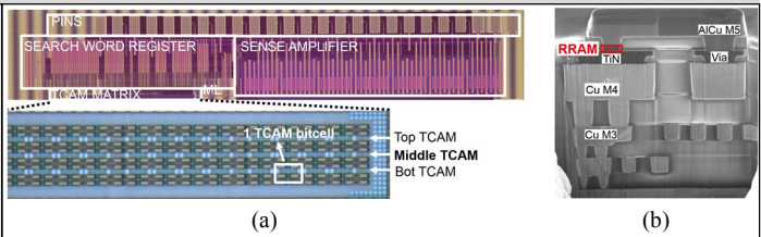
Fig.3: (a) Photo of the fabricated 1T2R1T TCAM circuit and (b) SEM cross-section of the integrated TiN/HfO 2 /Ti/TiN RRAM cells. Both HfO 2 and Ti layers are 10nm thick.
