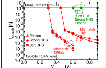
Fig.8: Measured search times, in case of match (green) and mismatch (red).
