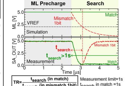
Fig.7: Waveforms of the search operation for a match (green) and mismatch (red). The search time is the time required to discharge the ML to VREF from the pre-charged value (VDD).
