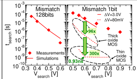
Fig.15: Measured (filled symbols) and simulated (lines) search times as a function of V_{search} . Search times can be improved by optimizing the sensing circuit ( \Delta V and MOS oxide thickness).
