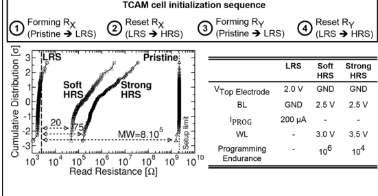
Fig.6: (top) TCAM cell initialization sequence and (bottom) RRAM pristine, LRS and HRS cumulative distributions with associated programming conditions. HRS distributions are obtained using the Soft HRS and Strong HRS programming conditions.
