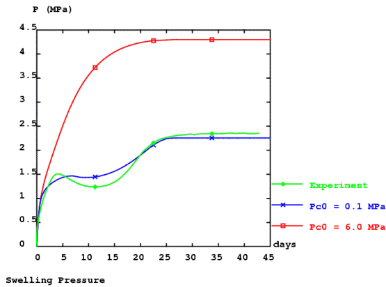
Figure 9. Swelling pressure obtained using roughly optimized parameters
