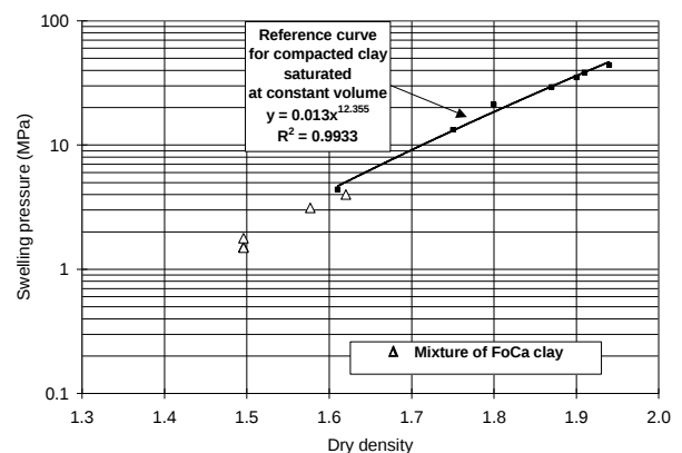
Figure 5. Swelling pressure versus dry density for a block compacted clay and for a mixture of powder and pellets.
