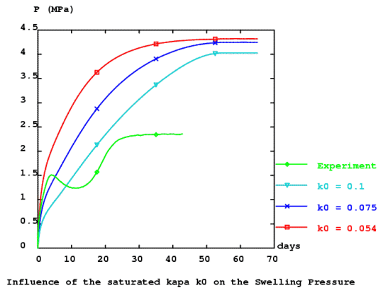
Figure 8. Variation of the swelling pressure with saturated stiffness \kappa_0 . Reference value is 0.054.
