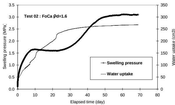
Figure 2. Evolution of the swelling pressure and water uptake versus time, mixture of FoCa clay, dry density 1.6 g/cm 3 .
