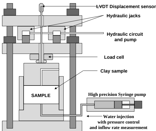
Figure 1. Schematic presentation of the experimental device.
