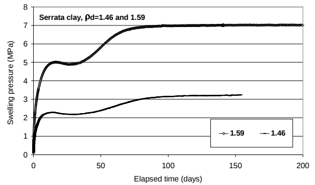
Figure 4. Evolution of the swelling pressure of 2 mixtures of powder and pellets of Serrata clay.
