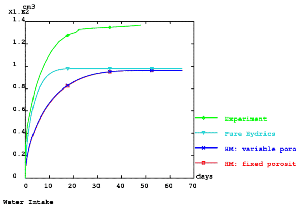
Figure 6. Total water absorbed by the sample. Experimental (diamond), constant porosity (inverse triangle) and coupled HM process (cross).
