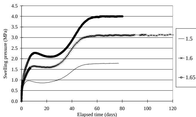
Figure 3. Swelling pressure of mixtures of pellets and powder of FoCa clay, for different dry densities.
