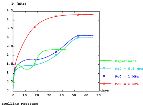
Figure 7. Swelling pressure versus time, using different preconsolidation levels P_{c0}^* . Reference value is 6 MPa.
