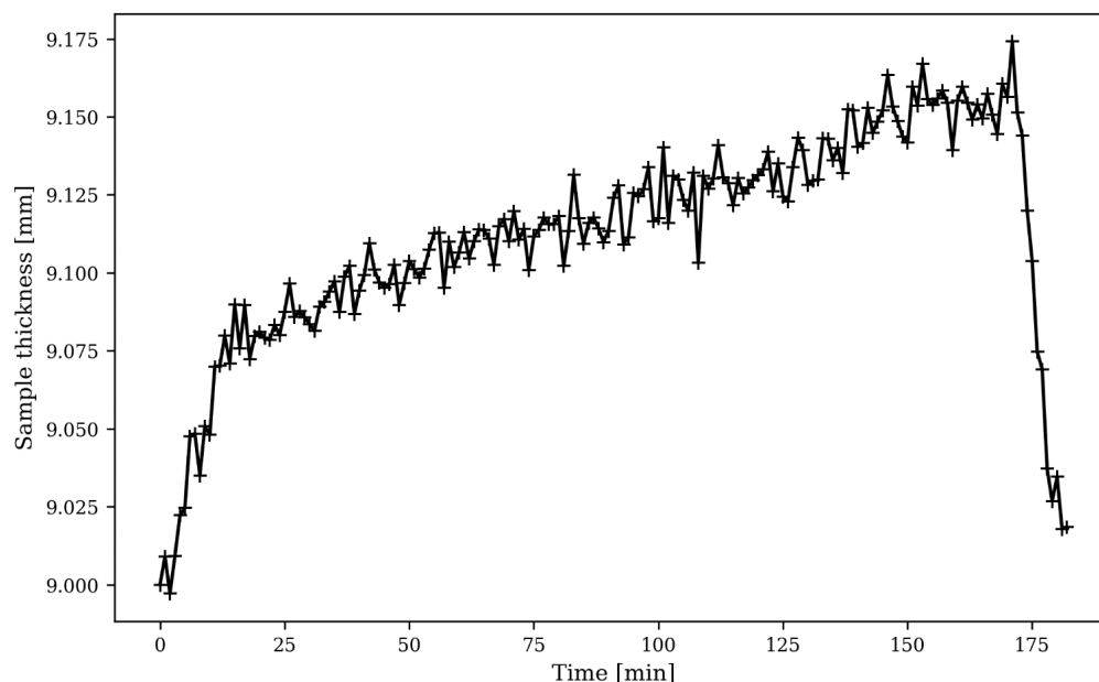
Fig. 4 : Swelling of a 2x2x9 mm standard MDF sample, placed in humid conditions at 90% RH and 25 °C for about three hours.
