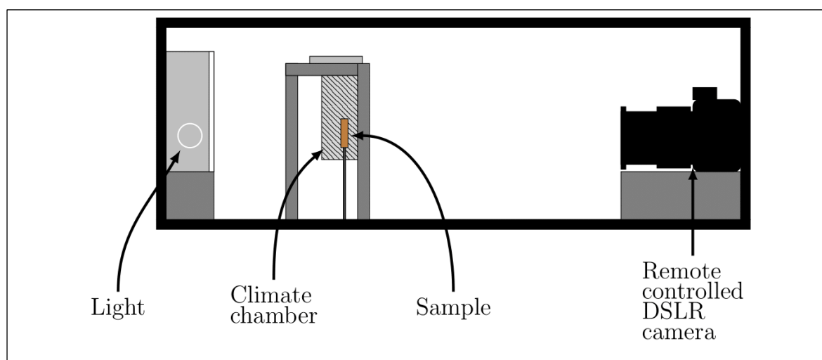
Fig. 3 : Photography setup, to acquire time-lapse videos of MDF swelling in a moist environment
