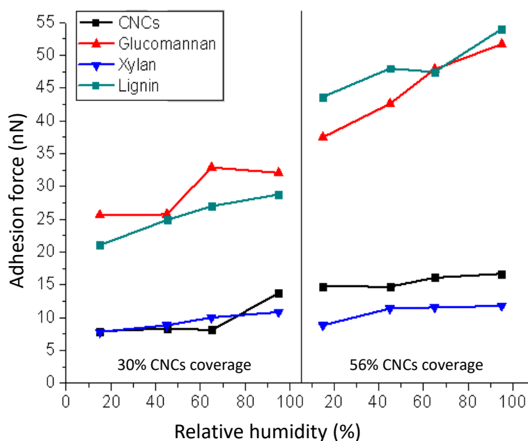
Fig. 2 : Effect of relative humidity on adhesion force between lignocellulosic films and CNCs at two CNCs coverage on the AFM lever (30 and 56%)
