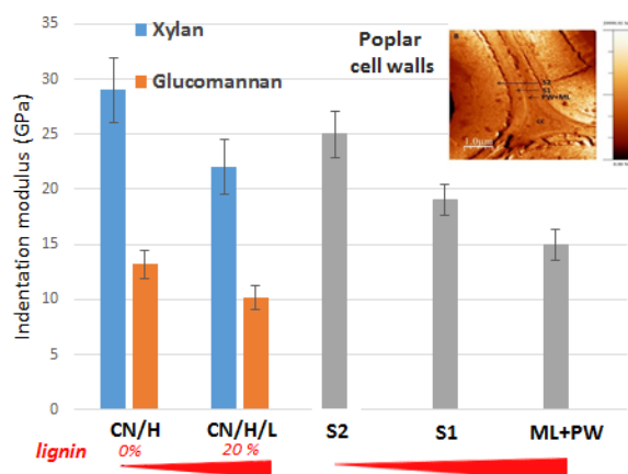
Fig. 1 : Impact of lignin on the indentation moduli of reconstituted films and the cell wall layers of poplar fibre
