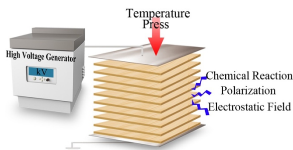
Fig. 1 : Schematic diagram showing the high voltage generator applied in the LVL.
