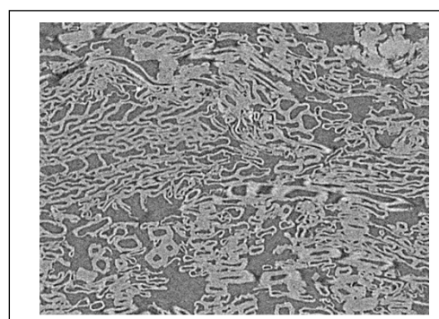
Fig. 2 : Cross-section of a high resolution (voxel size 500nm) scan of MDF
