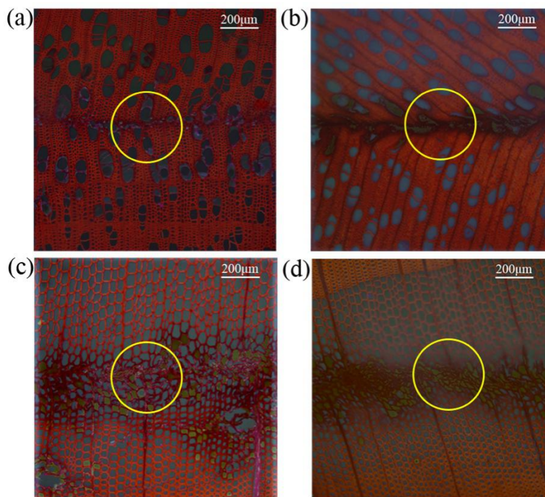
Fig. 2 : Micrographs of (a) untreated Poplar LVL bonding interphase compared with (b) treated one. Micrographs of (c) untreated Masson pine LVL compared with (d) treated one.
